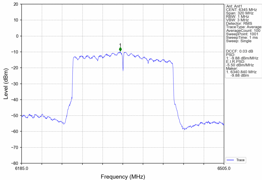
802.11ax(HEW160)_HCH_6345MHz_2xRU996_Left_Ant1_NTNV
