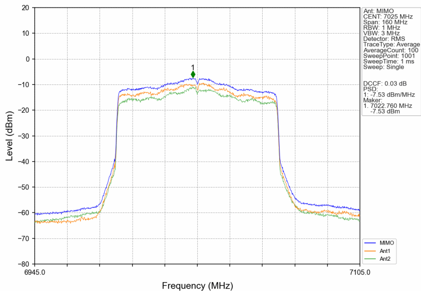
802.11ax(HEW80)_HCH_7025MHz_RU996_Left_MIMO_NTNV
