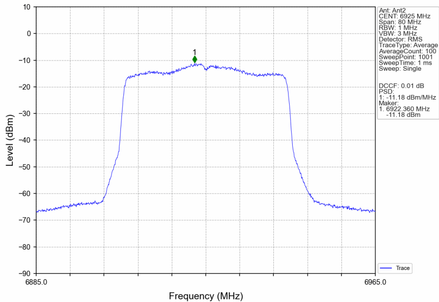
802.11ax(HEW40)_LCH_6925MHz_RU484_Left_MIMO_NTNV
