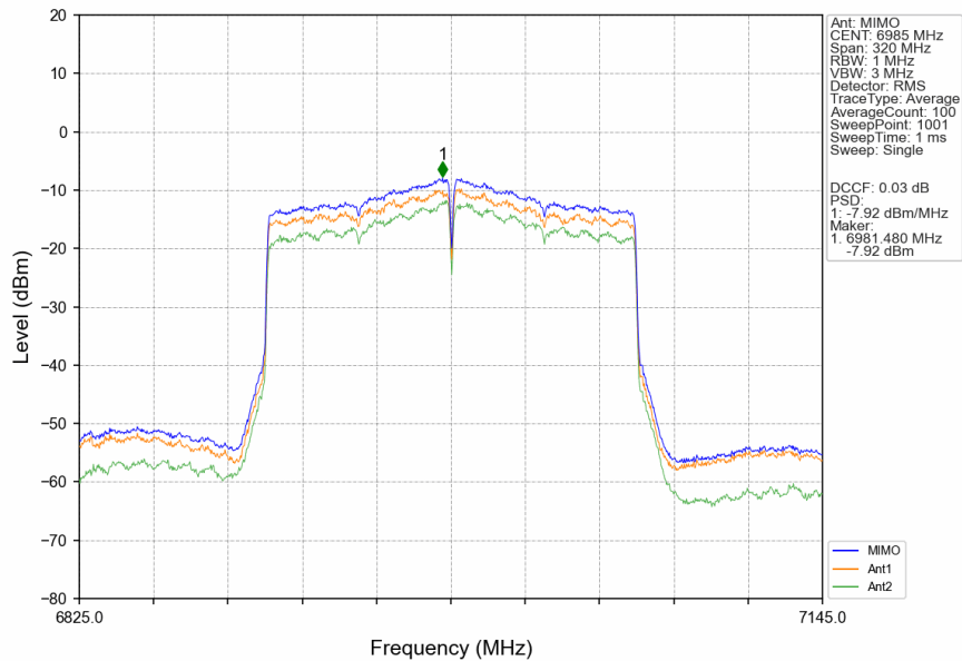
802.11ax(HEW160)_MCH_6985MHz_2xRU996_Left_MIMO_NTNV
