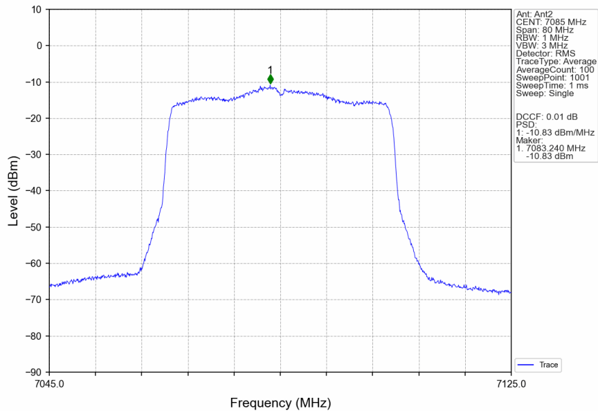
802.11ax(HEW40)_HCH_7085MHz_RU484_Left_MIMO_NTNV
