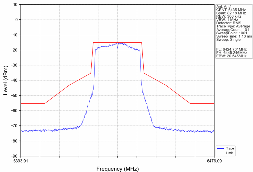
802.11ax(HEW20)_LCH_6435MHz_RU242_Left_Ant1_NTNV
