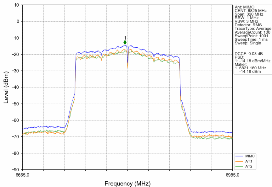
802.11ax(HEW160)_HCH_6825MHz_2xRU996_Left_MIMO_NTNV
