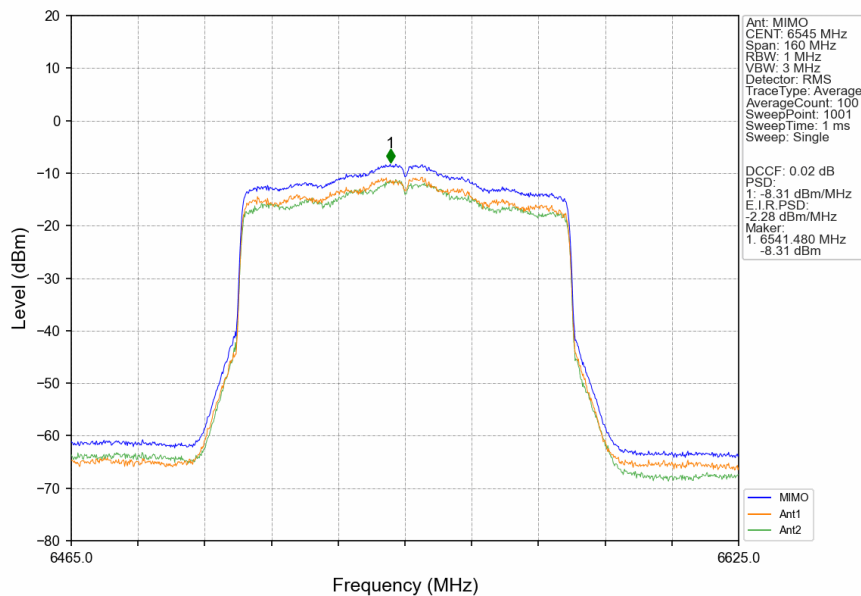
802.11ax(HEW80)_HCH_6545MHz_RU996_Left_MIMO_NTNV
