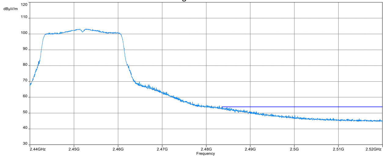
Average Detector
