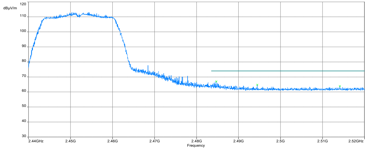
Peak Detector
