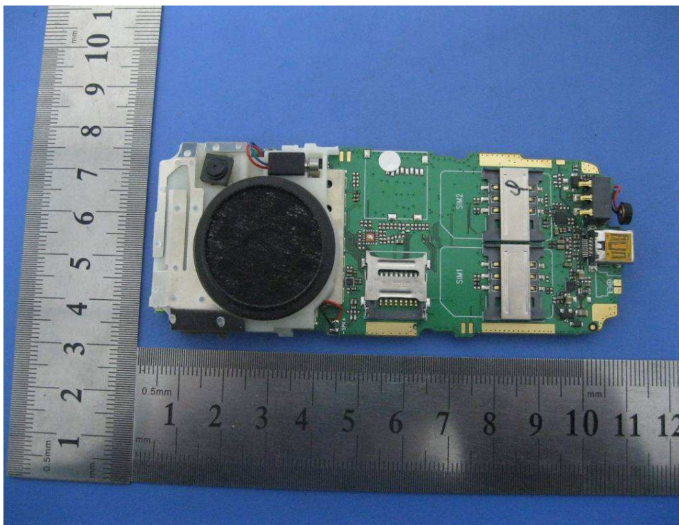
EUT – Main Board Top View
