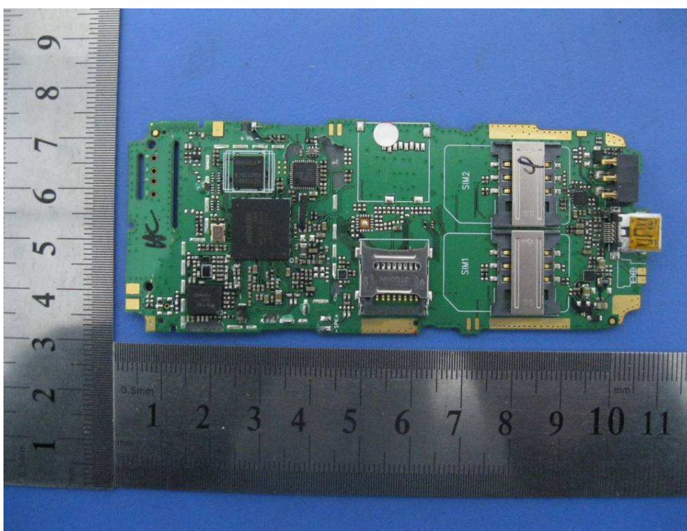
EUT – Main Board Shielding off Top View
