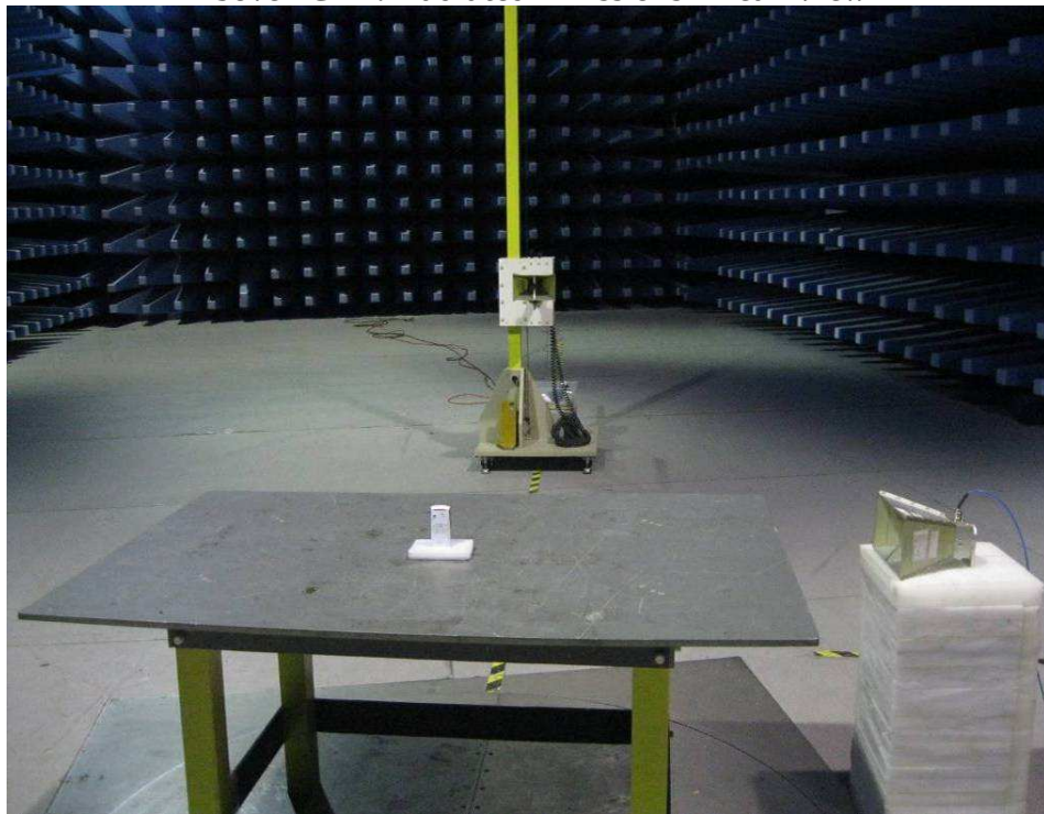
Above 1GHz: Radiated Emissions - Rear View
