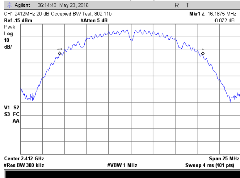
Channel 1 (20 dB)
