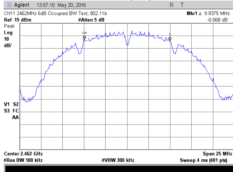
Channel 11 (6 dB)
