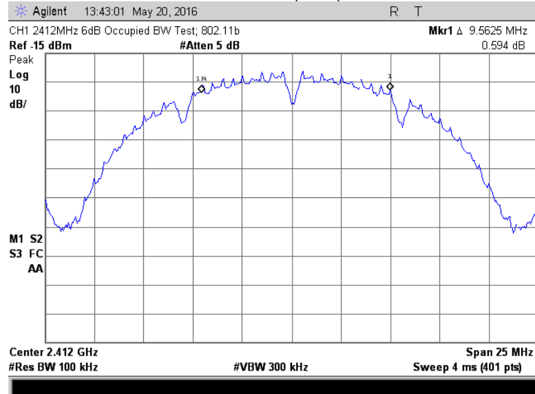
Channel 1 (6 dB)
