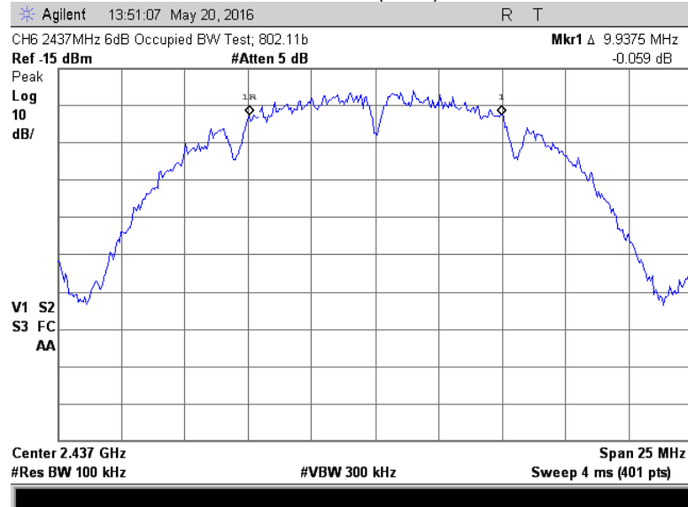
Channel 6 (6 dB)
