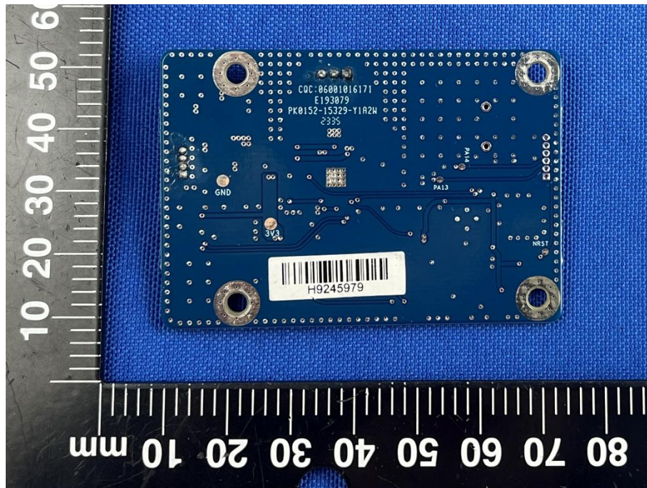
SECONDARY BOARD 4 REAR VIEW (RFID-2)
