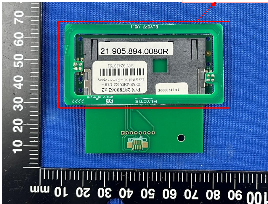
SECONDARY BOARD 5 REAR VIEW (RFID-3)
