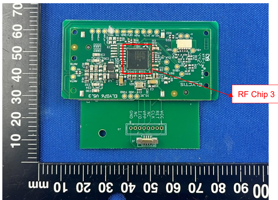
SECONDARY BOARD 5 TOP VIEW (RFID-3)
