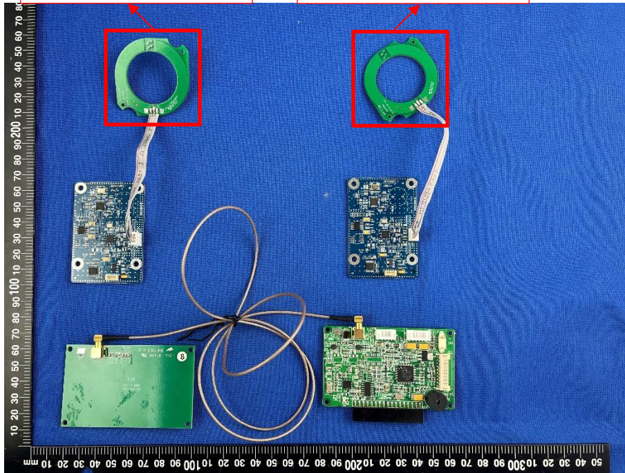
Coil Antenna (RFID 1)
