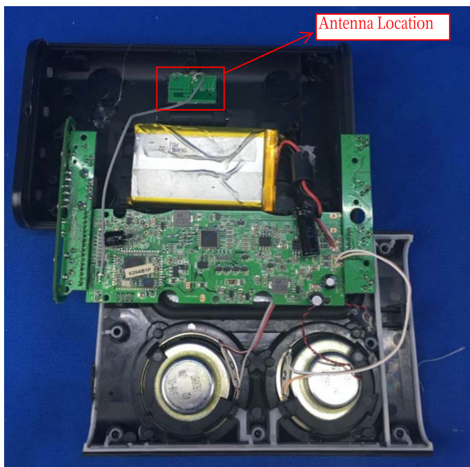
INTERNAL PHOTO OF SAMPLE-4
