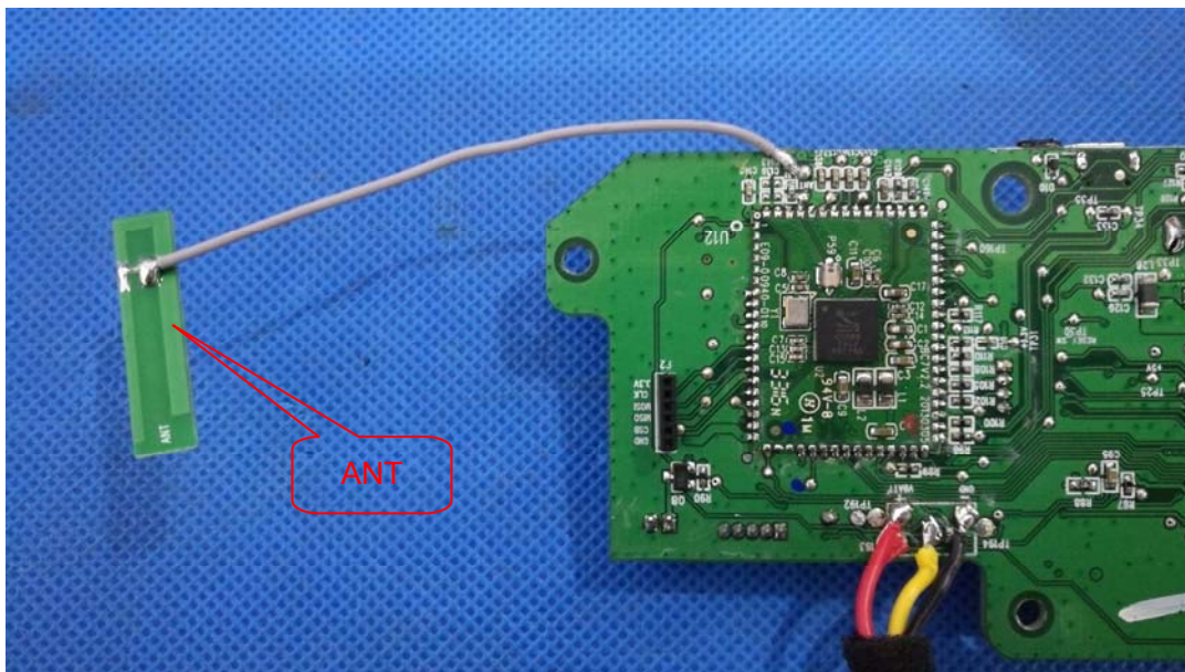
Antenna RF Port
