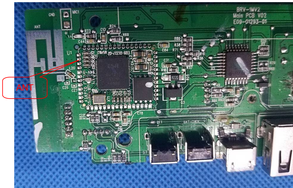
Antenna RF Port
