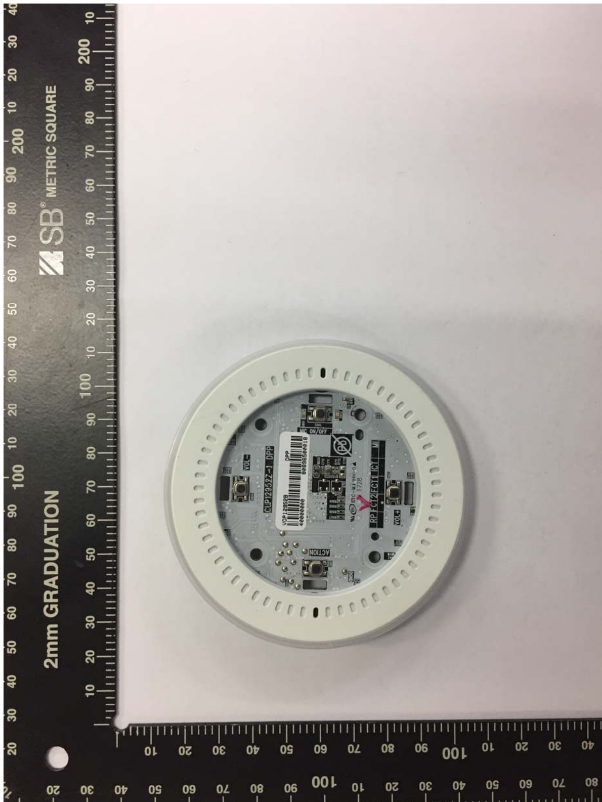
Front View of ASR board
