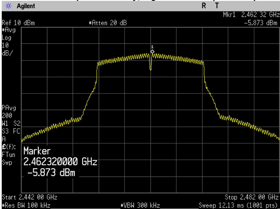
Maximum Power Spectral Density, Highest Channel (2462 MHz)
