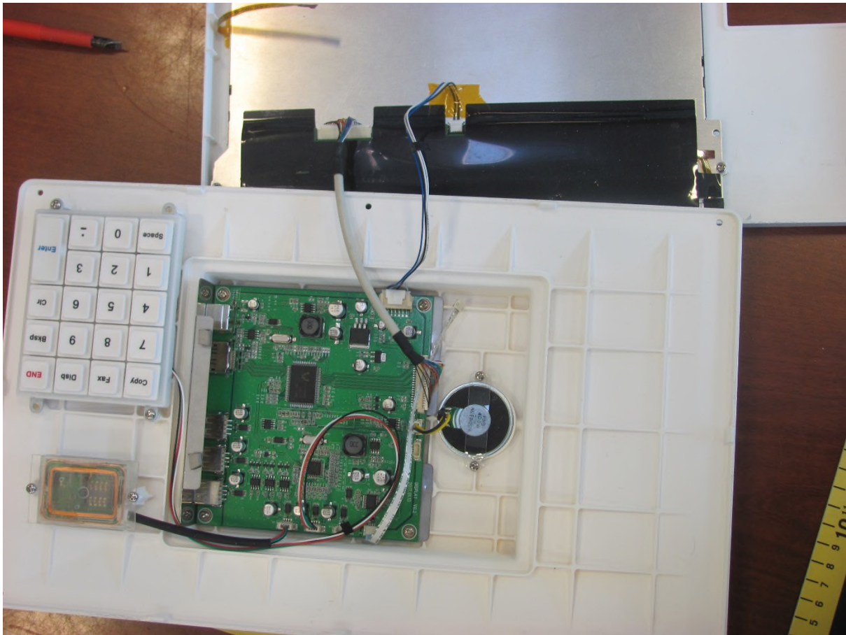
Figure 2 – EUT Internal Photo - Monitor
