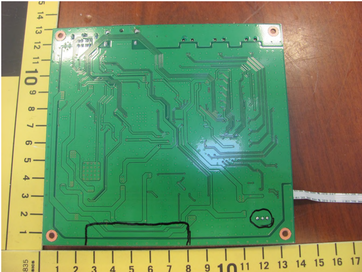
Figure 4 – EUT Internal Photo – Monitor PCB bottom view
