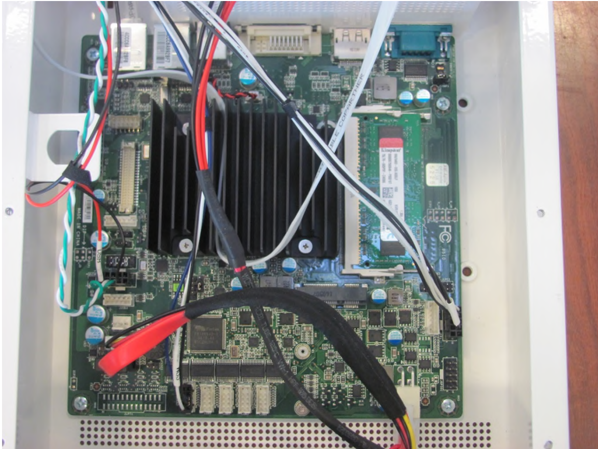
Figure 1 – EUT Internal Photo – Edge PC
