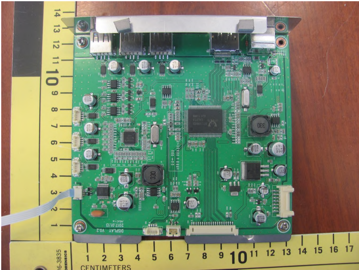
Figure 3 – EUT Internal Photo – Monitor PCB top view
