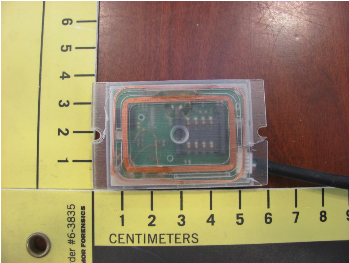
Figure 6 – EUT Internal Photo – Transmitter bottom view
