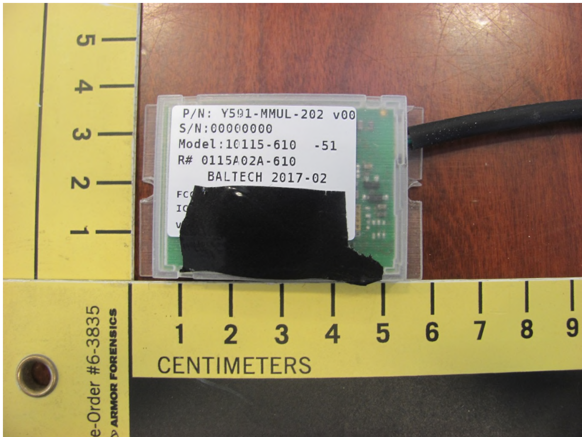
Figure 5 – EUT Internal Photo – Transmitter top view
