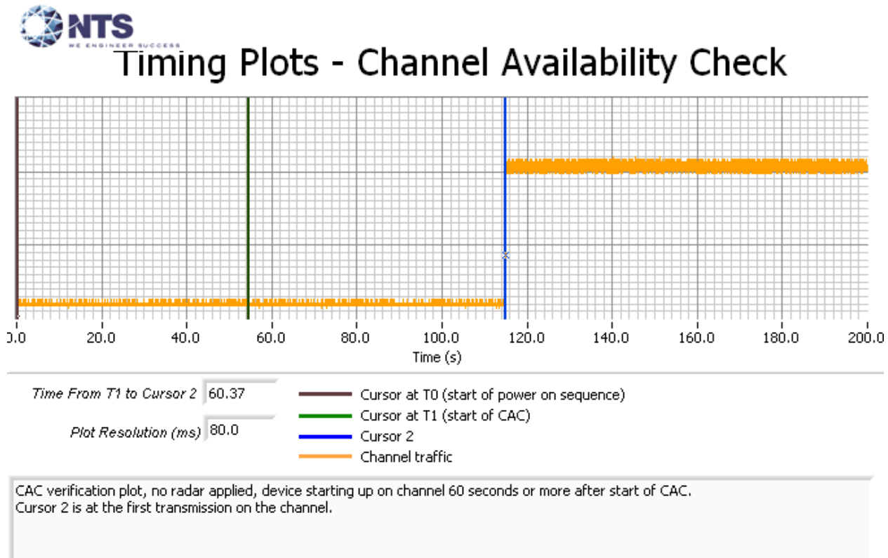
Figure 18 Plot of EUT Start-Up after CAC
