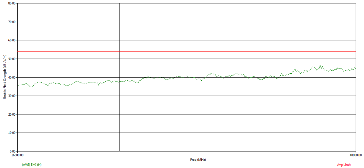
Figure 90: Average RE from 26.5GHz to 40GHz - Horizontal polarization
