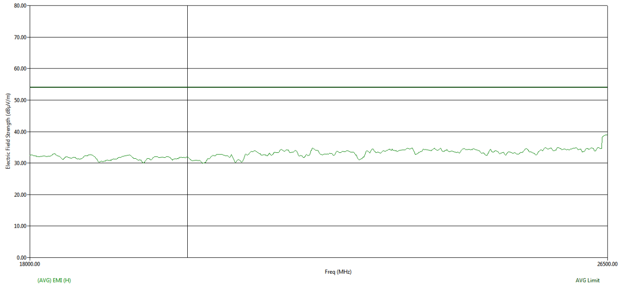
Figure 108: Average RE from 18GHz to 26.5GHz - Horizontal polarization
