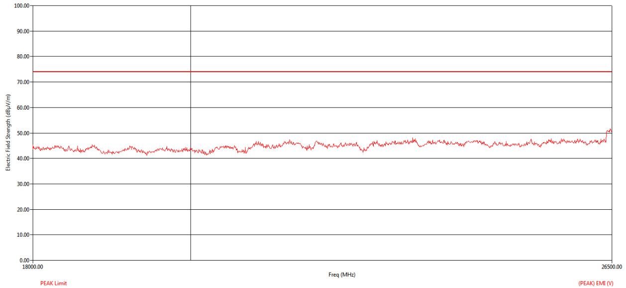
Figure 67: Peak RE from 18GHz to 26.5GHz - Vertical polarization
