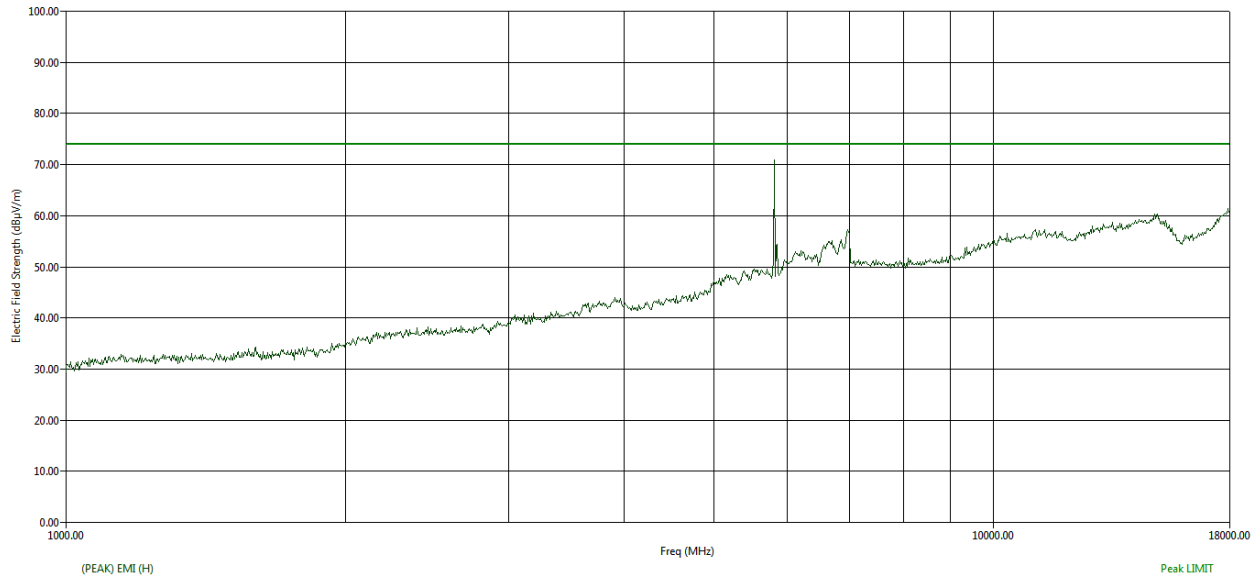
Figure 84: Peak RE from 1GHz to 18GHz - Horizontal polarization
