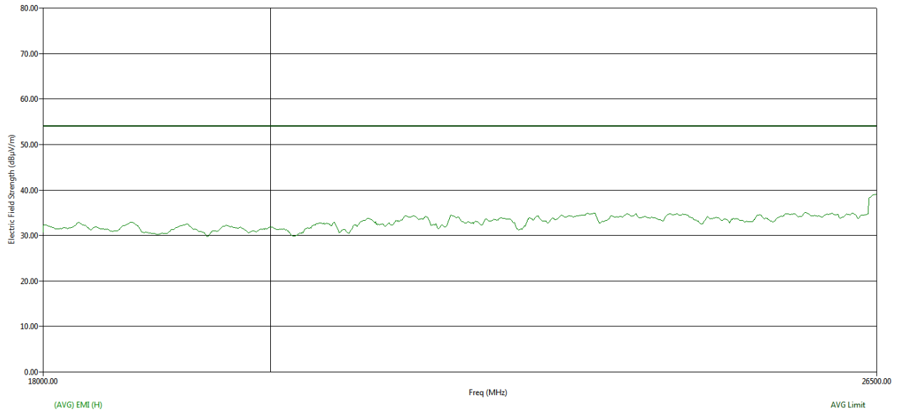
Figure 86: Average RE from 18GHz to 26.5GHz - Horizontal polarization
