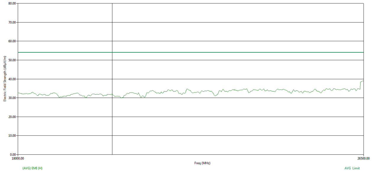
Figure 130: Average RE from 18GHz to 26.5GHz - Horizontal polarization
