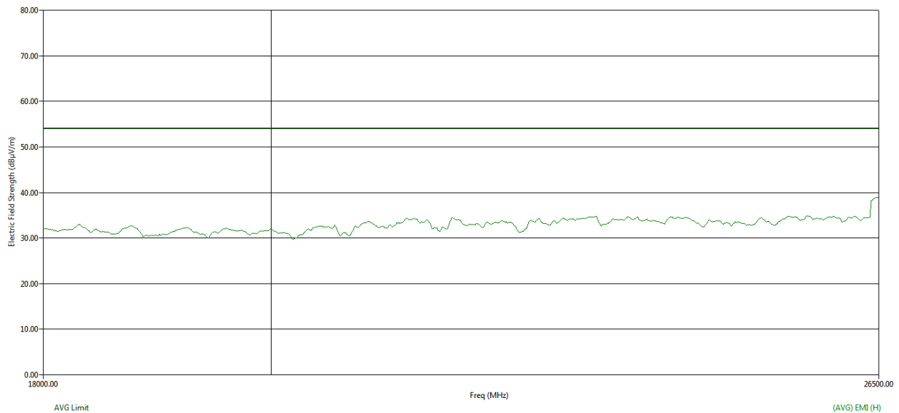
Figure 42: Average RE from 18GHz to 26.5GHz - Horizontal polarization
