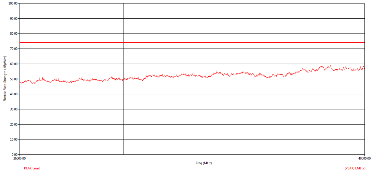
Figure 49: Peak RE from 26.5GHz to 40GHz - Vertical polarization
