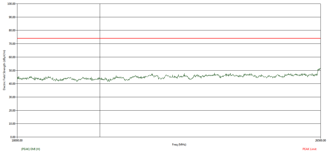
Figure 44: Peak RE from 18GHz to 26.5GHz - Horizontal polarization
