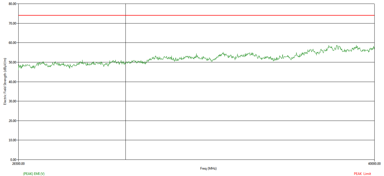
Figure 137: Peak RE from 26.5GHz to 40GHz - Vertical polarization
