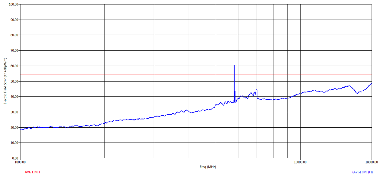
Figure 82: Average RE from 1GHz to 18GHz - Horizontal polarization
