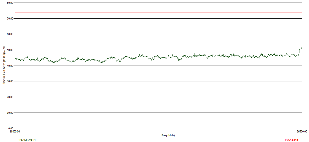
Figure 88: Peak RE from 18GHz to 26.5GHz - Horizontal polarization
