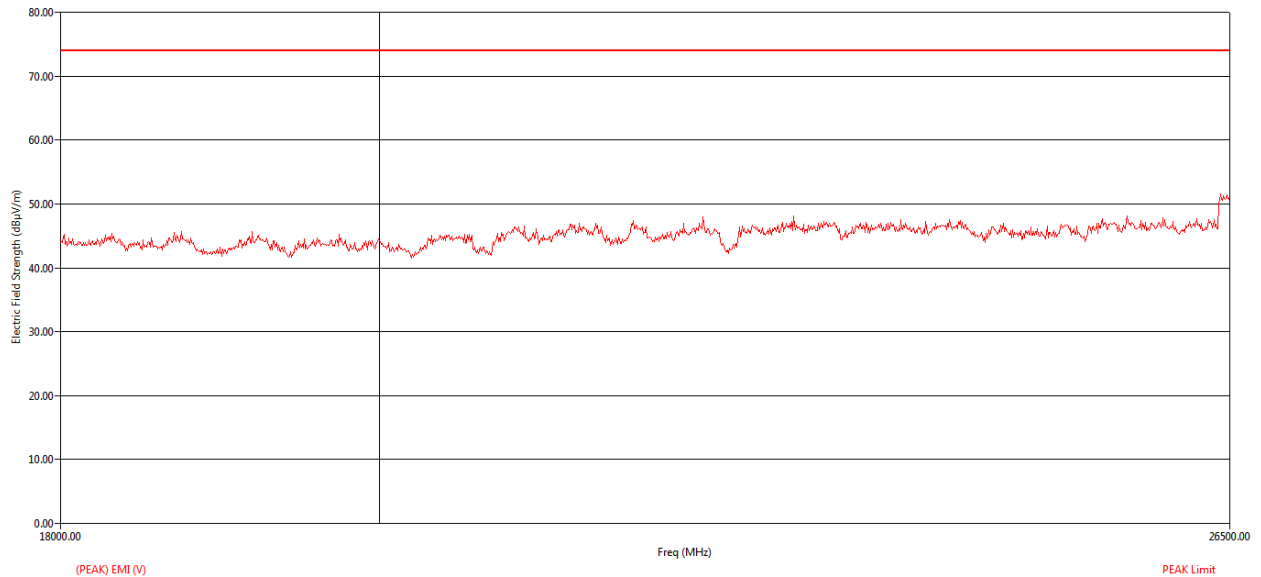
Figure 133: Peak RE from 18GHz to 26.5GHz - Vertical polarization
