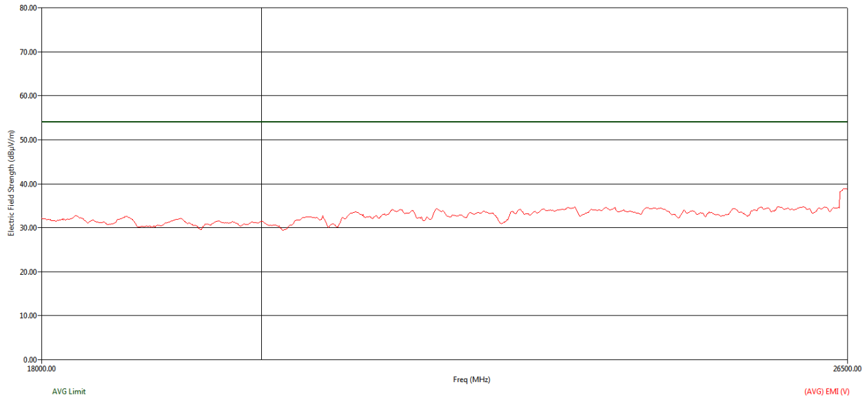
Figure 43: Average RE from 18GHz to 26.5GHz - Vertical polarization
