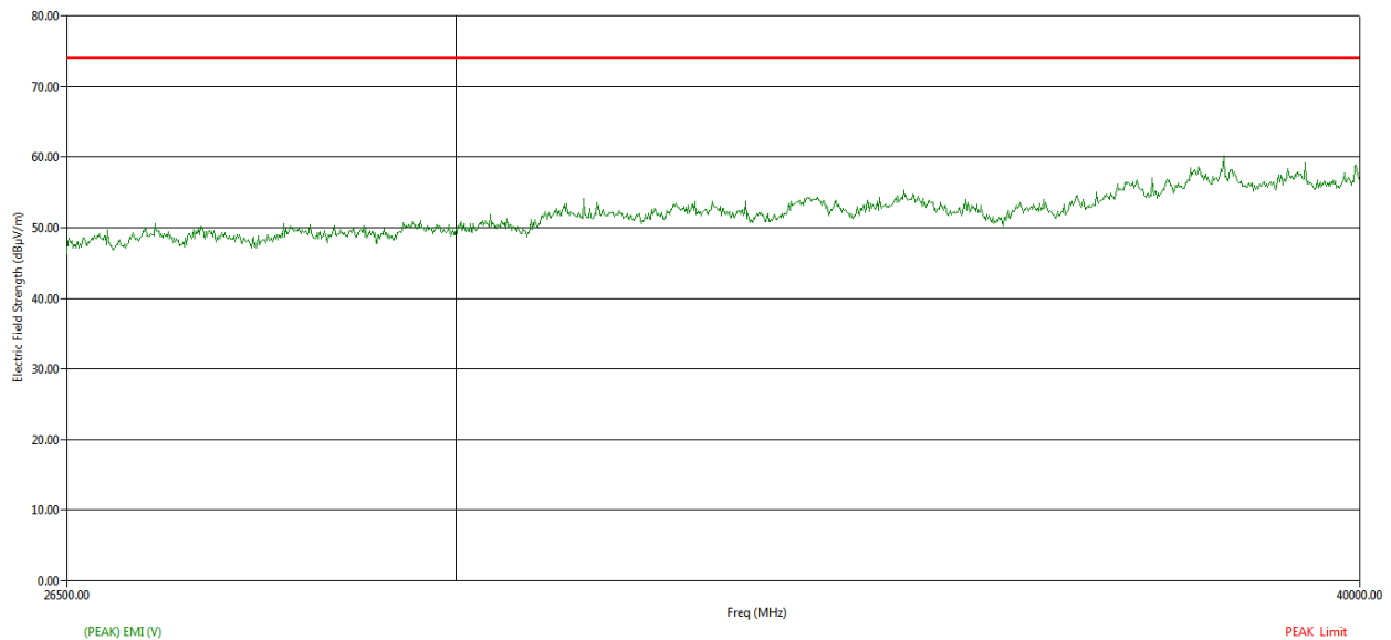
Figure 93: Peak RE from 26.5GHz to 40GHz - Vertical polarization
