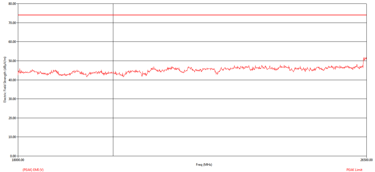
Figure 89: Peak RE from 18GHz to 26.5GHz - Vertical polarization
