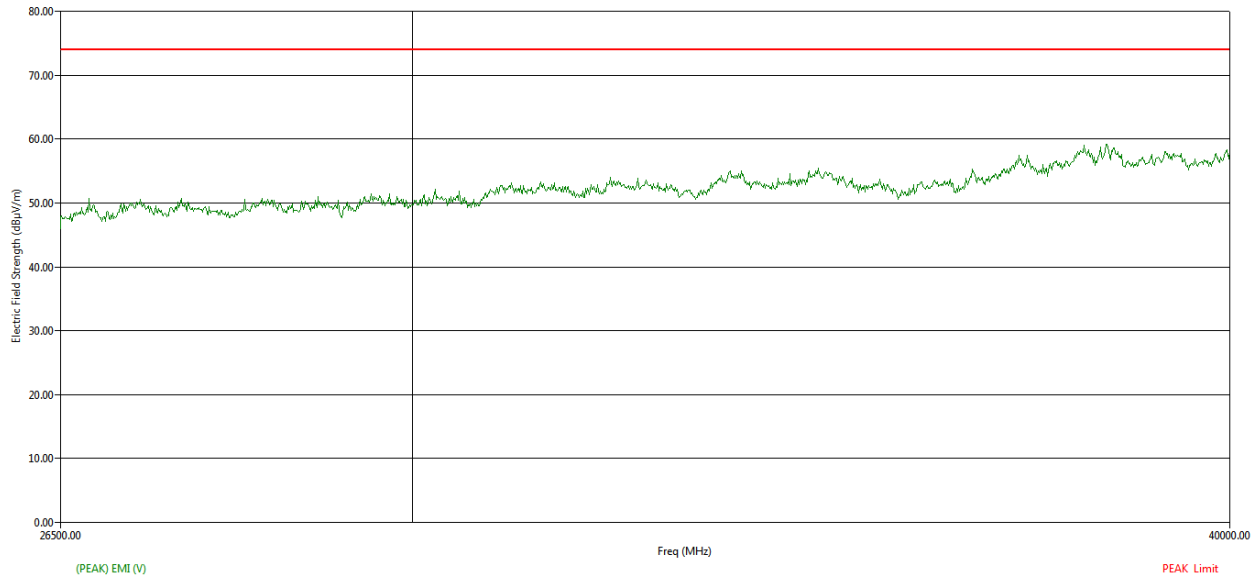
Figure 71: Peak RE from 26.5GHz to 40GHz - Vertical polarization
