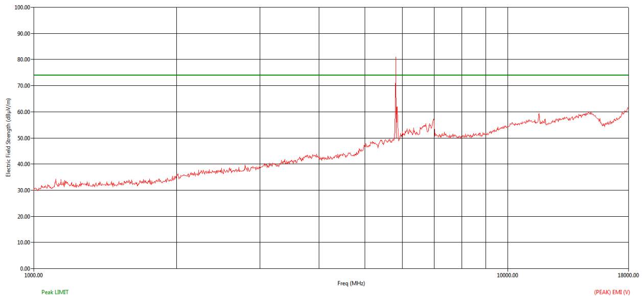
Figure 151: Peak RE from 1GHz to 18GHz - Vertical polarization
