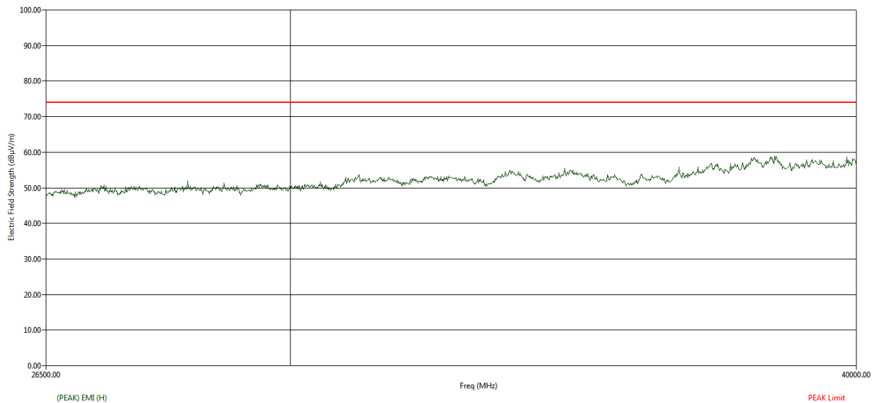
Figure 48: Peak RE from 26.5GHz to 40GHz - Horizontal polarization
