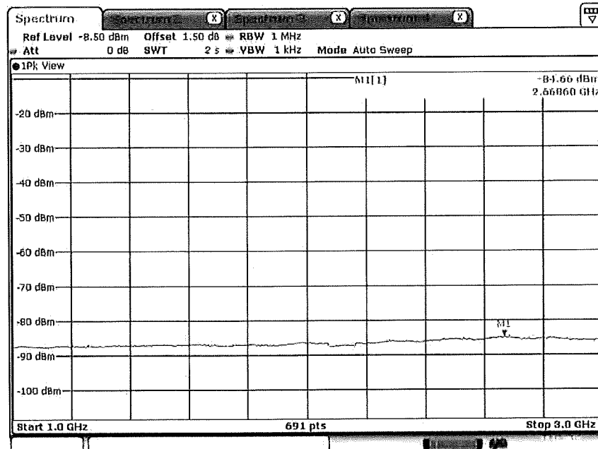
Plot on Configuration QPSK, 20M / 5745 MHz / Average / Port 2 / 1GHz~3GHz
