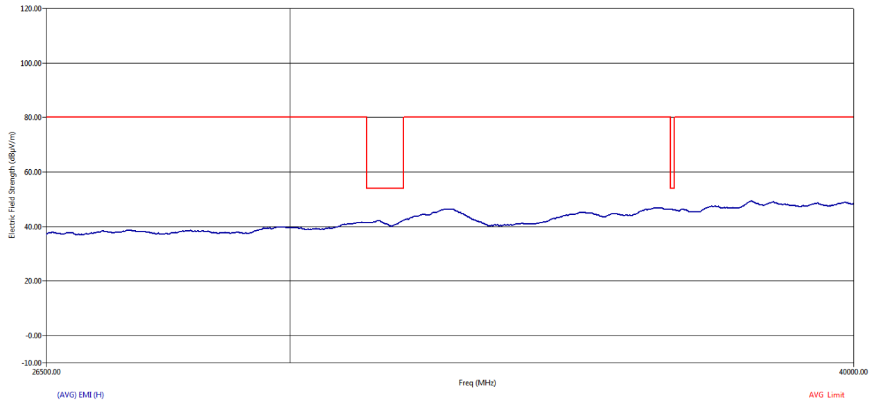
Figure 109 RE Graph from 26.5 GHz to 40 GHz using Average Detector – Horizontal Polarization
