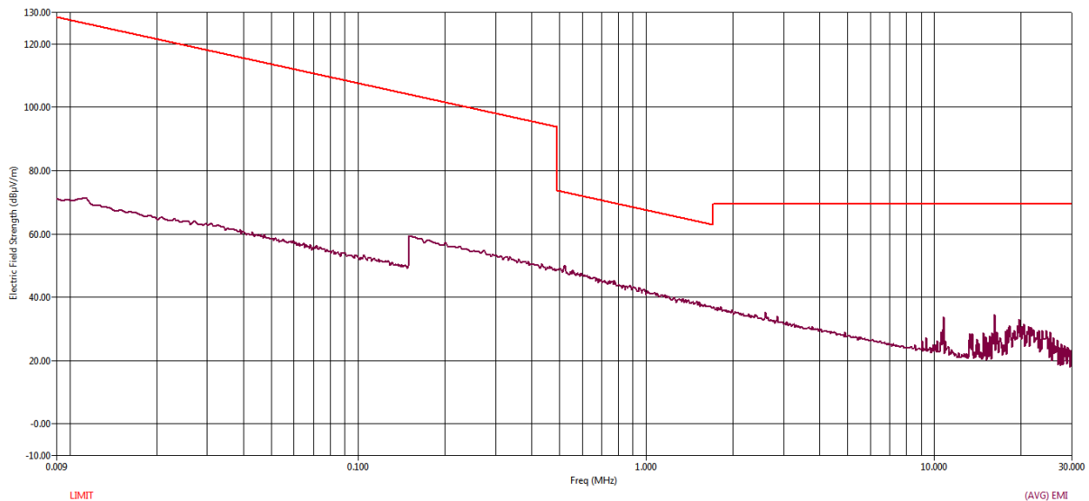
Figure 138 RE Graph from 9 kHz to 30 MHz using Average Detector – Perpendicular
