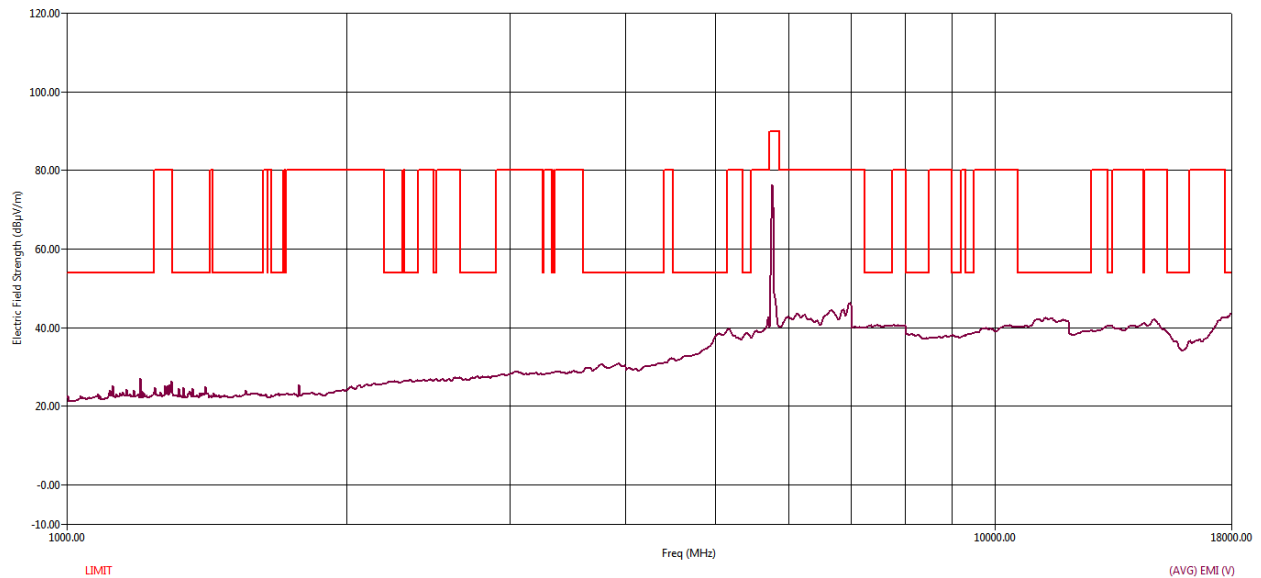
Figure 82 RE Graph from 1 GHz to 18 GHz using Average Detector – Vertical Polarization
