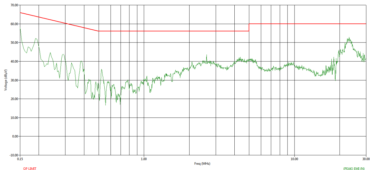
Figure 160 CE graph from 150 kHz to 30 MHz using Peak detector-Neutral
