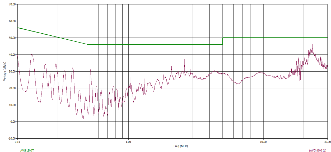
Figure 163 CE graph from 150 kHz to 30 MHz using Average detector – Line
