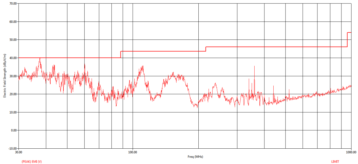
Figure 104 RE Graph from 30 MHz to 1 GHz using Peak Detector – Vertical Polarization
