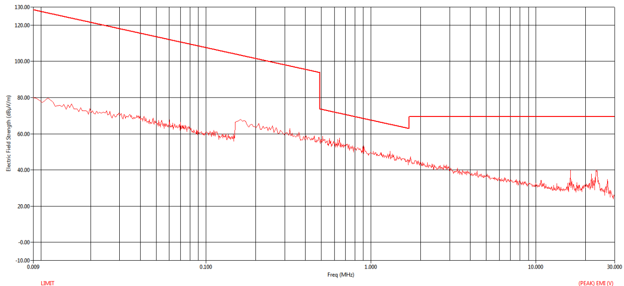
Figure 29 RE Graph from 9 kHz to 30 MHz using Peak Detector – Perpendicular
