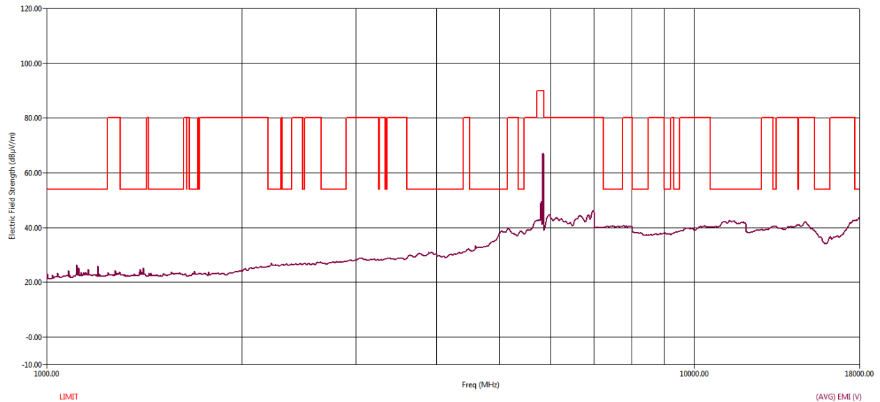
Figure 142 RE Graph from 1 GHz to 18 GHz using Average Detector – Vertical Polarization
