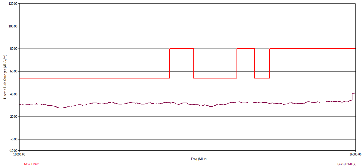
Figure 36 RE Graph from 18 GHz to 26.5 GHz using Average detector – Vertical Polarization
