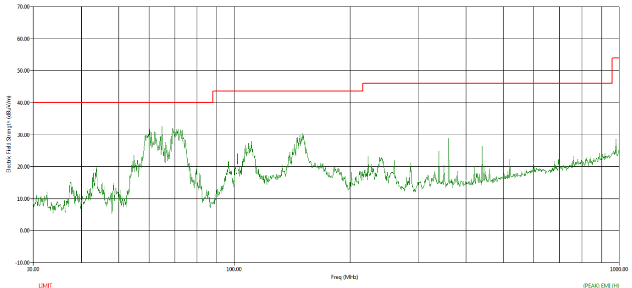
Figure 127 RE Graph from 30 MHz to 1 GHz using Peak Detector – Horizontal Polarization
