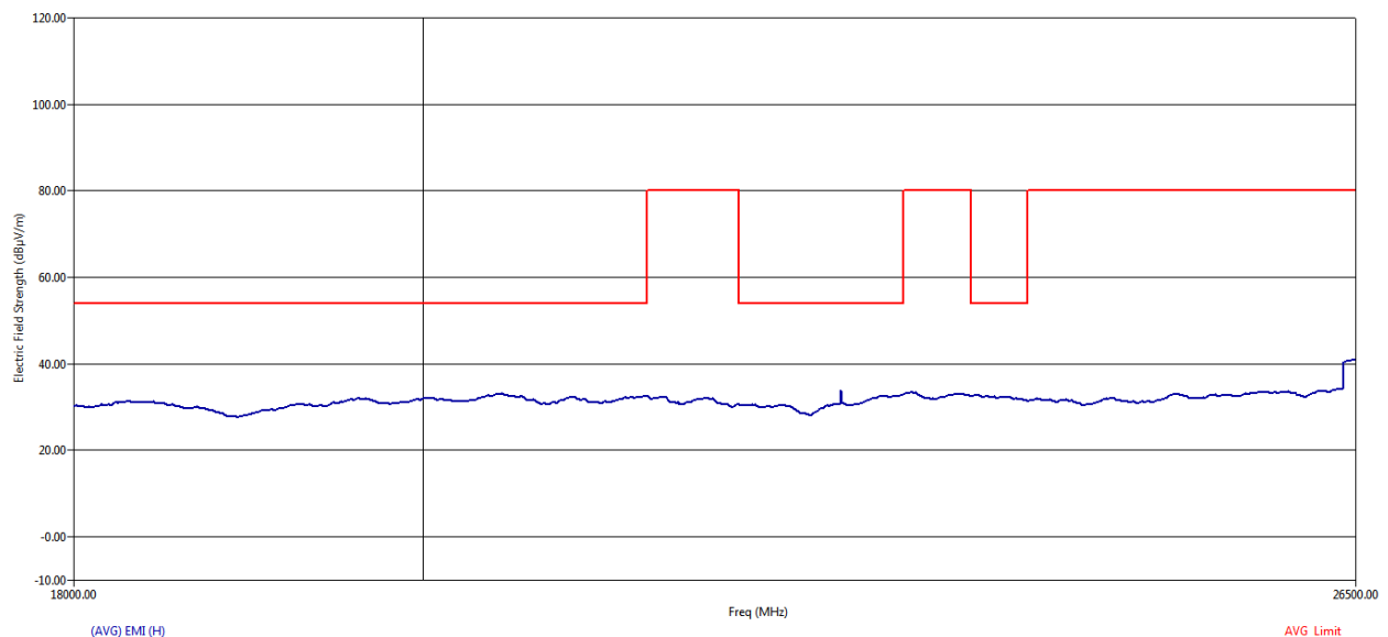
Figure 23 RE Graph from 18 GHz to 26.5 GHz using Average detector – Horizontal Polarization
