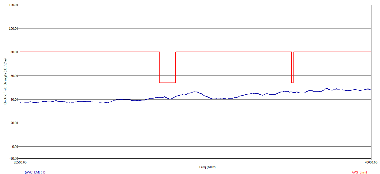
Figure 25 RE Graph from 26.5 GHz to 40 GHz using Average detector – Horizontal Polarization
