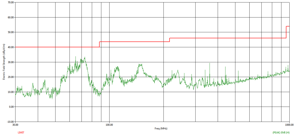
Figure 103 RE Graph from 30 MHz to 1 GHz using Peak Detector – Horizontal Polarization
