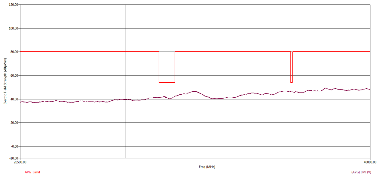
Figure 110 RE Graph from 26.5 GHz to 40 GHz using Average Detector – Vertical Polarization
