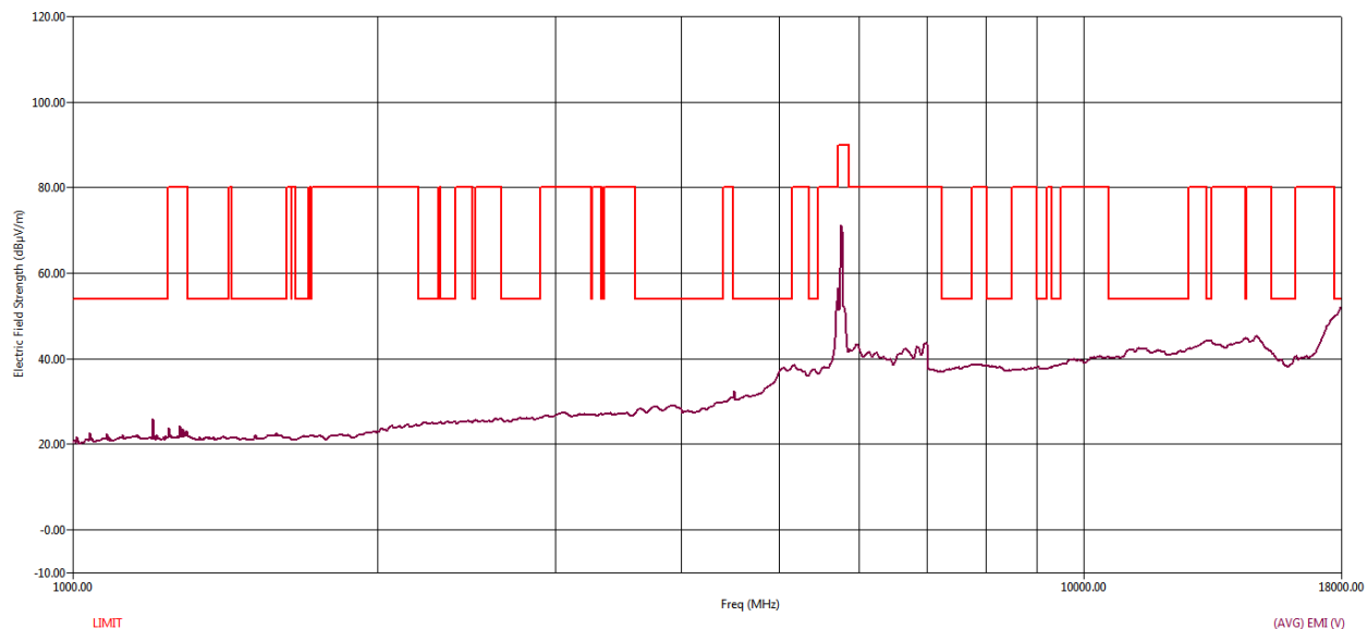
Figure 10 RE Graph from 1 GHz to 18 GHz using Average detector – Vertical Polarization
