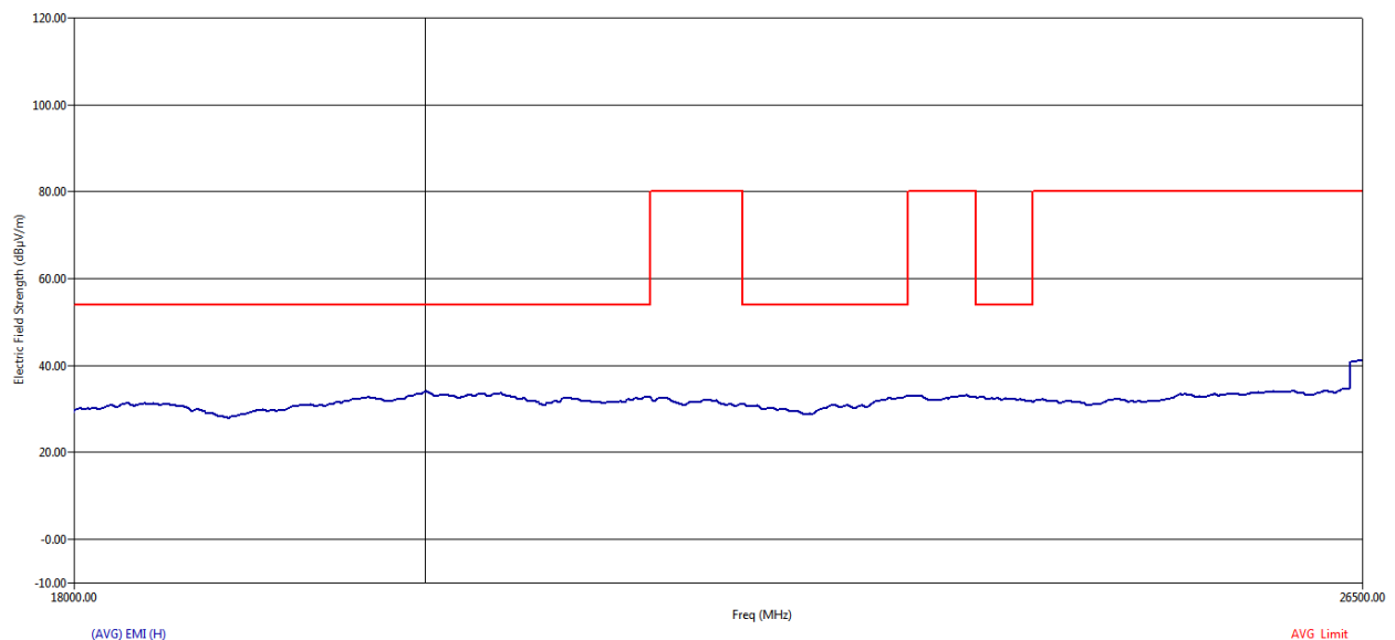
Figure 143 RE Graph from 18 GHz to 26.5 GHz using Average Detector – Horizontal Polarization
