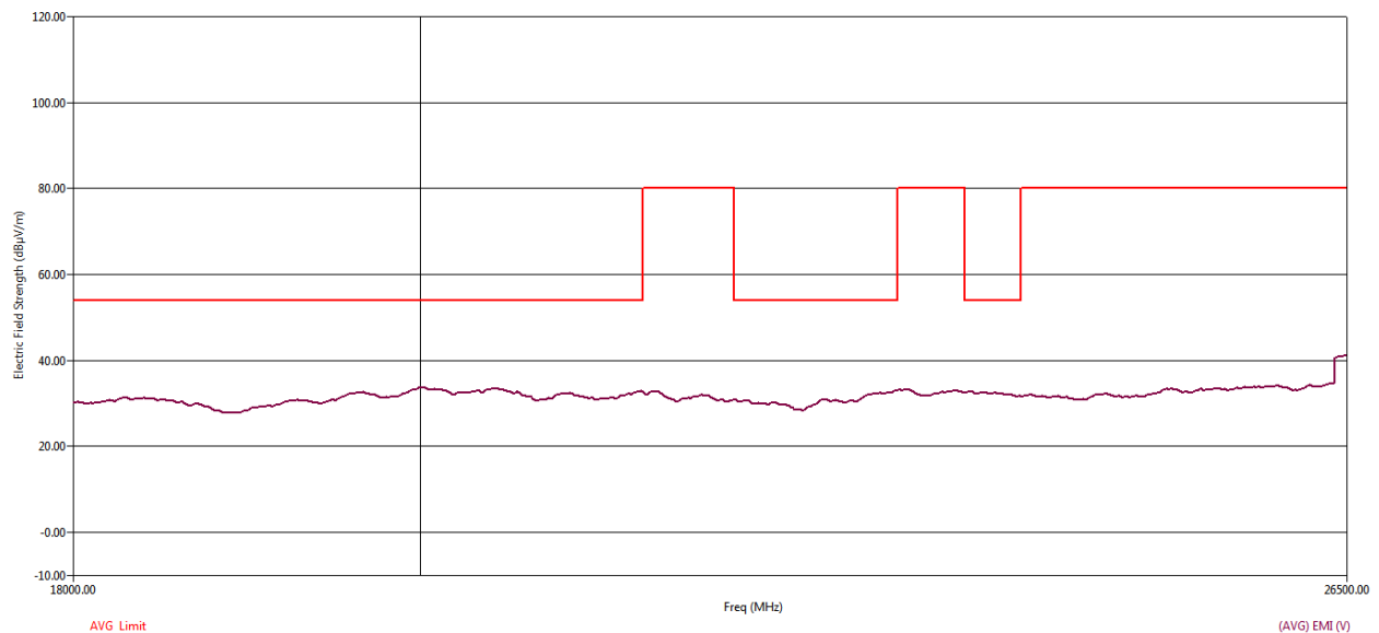
Figure 60 RE Graph from 18 GHz to 26.5 GHz using Average detector – Vertical Polarization
