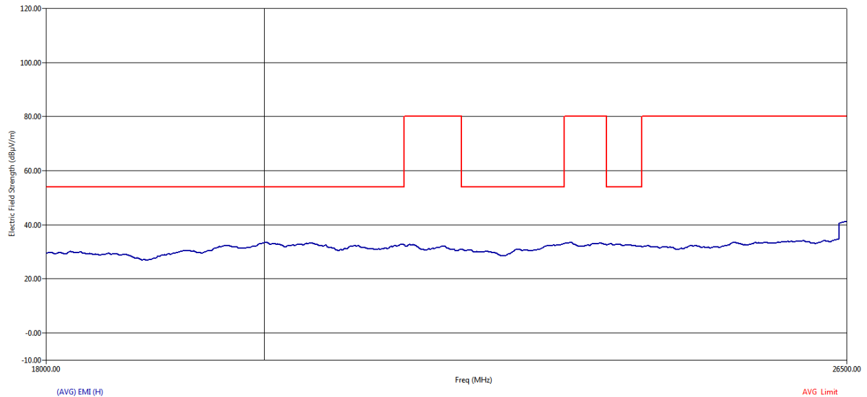
Figure 119 RE Graph from 18 GHz to 26.5 GHz using Average Detector – Horizontal Polarization
