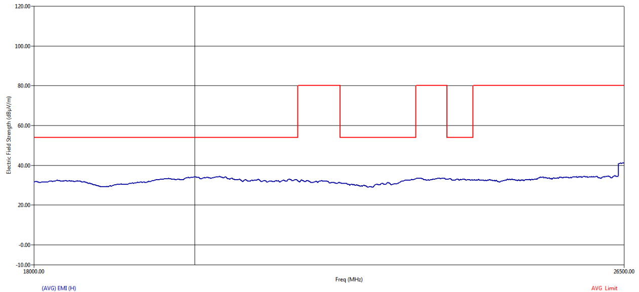
Figure 107 RE Graph from 18 GHz to 26.5 GHz using Average Detector – Horizontal Polarization
