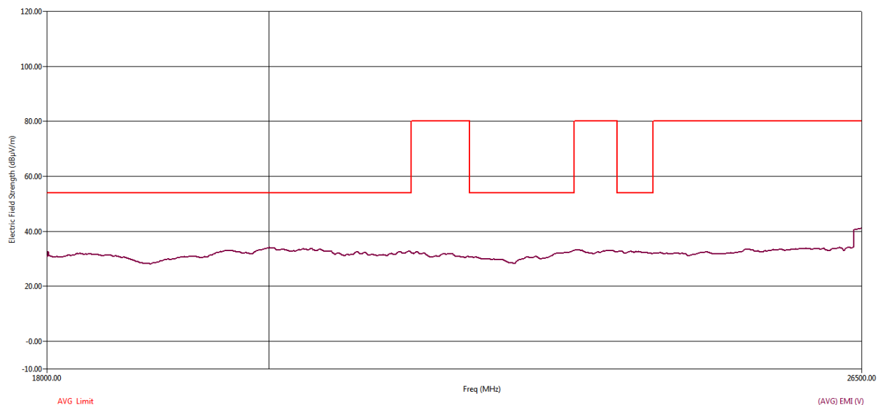
Figure 84 RE Graph from 18 GHz to 26.5 GHz using Average Detector – Vertical Polarization
