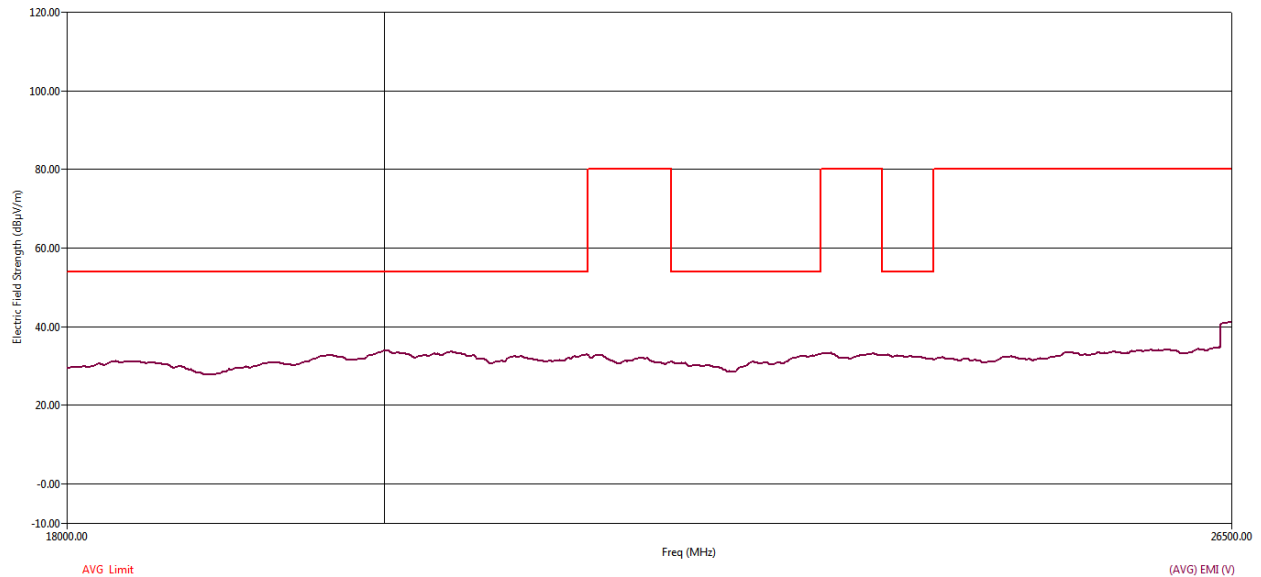
Figure 144 RE Graph from 18 GHz to 26.5 GHz using Average Detector – Vertical Polarization
