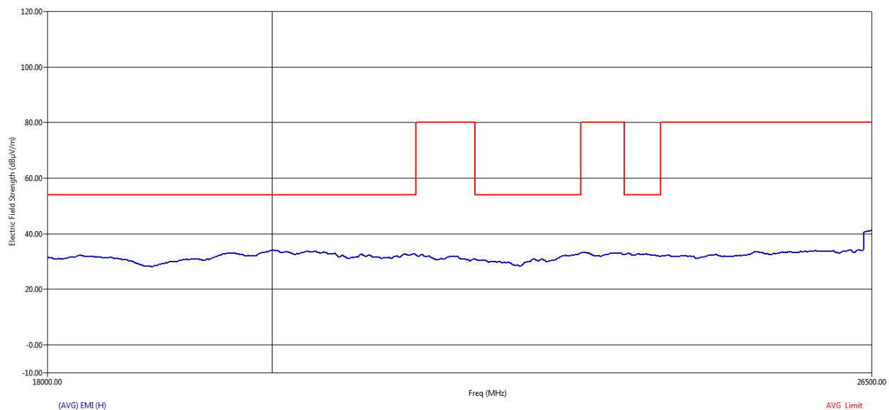
Figure 95 RE Graph from 18 GHz to 26.5 GHz using Average Detector – Horizontal Polarization
