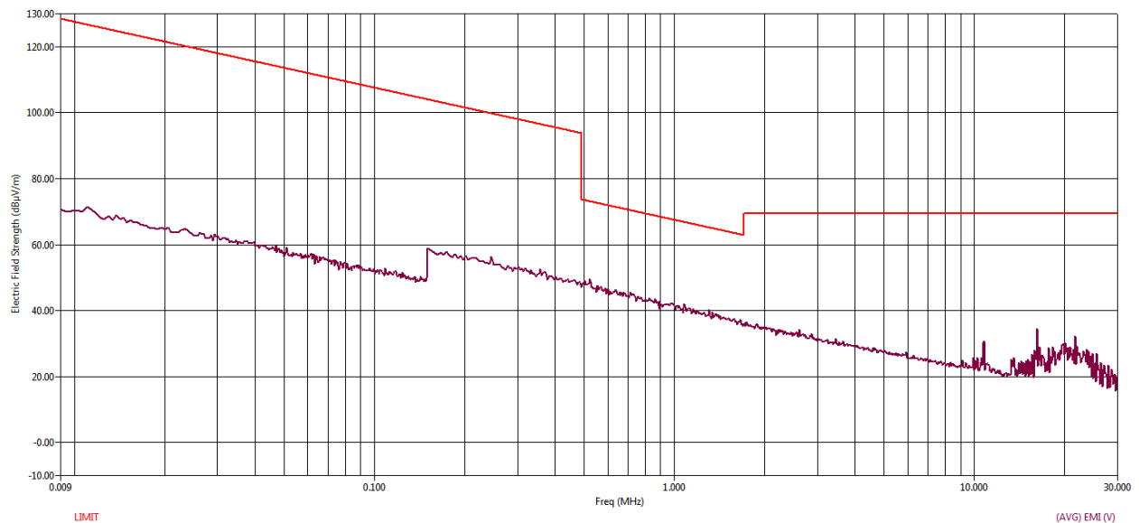
Figure 90 RE Graph from 9 kHz to 30 MHz using Average Detector – Perpendicular
