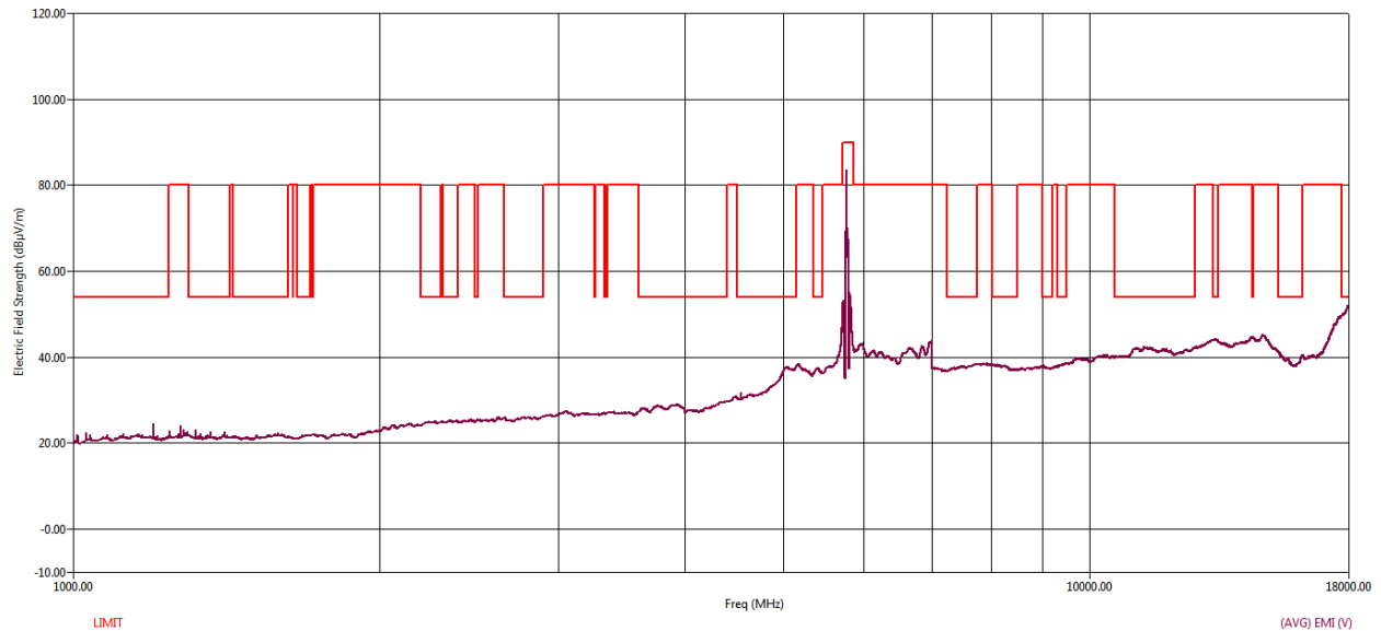
Figure 22 RE Graph from 1 GHz to 18 GHz using Average detector –Vertical Polarization
