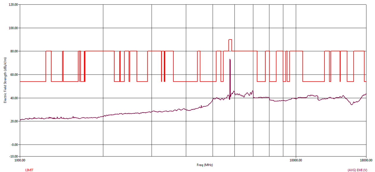
Figure 58 RE Graph from 1 GHz to 18 GHz using Average detector – Vertical Polarization
