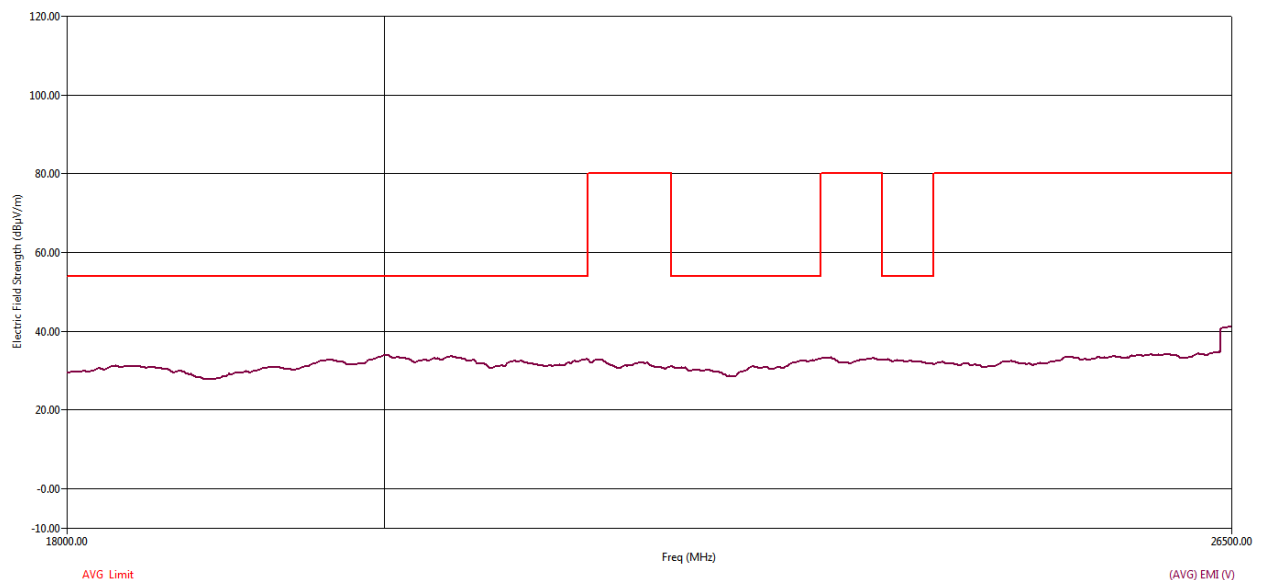
Figure 72 RE Graph from 18 GHz to 26.5 GHz using Average detector – Vertical Polarization
