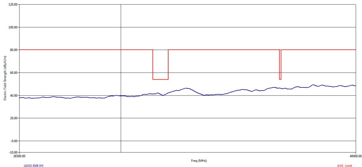
Figure 49 RE Graph from 26.5 GHz to 40 GHz using Average detector – Horizontal Polarization
