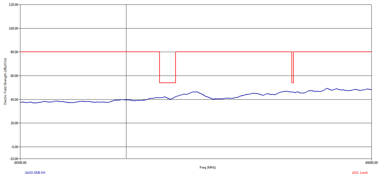
Figure 97 RE Graph from 26.5 GHz to 40 GHz using Average Detector – Horizontal Polarization
