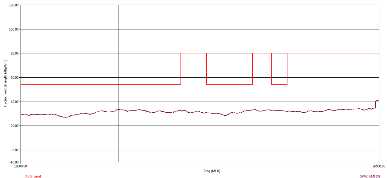
Figure 120 RE Graph from 18 GHz to 26.5 GHz using Average Detector – Vertical Polarization
