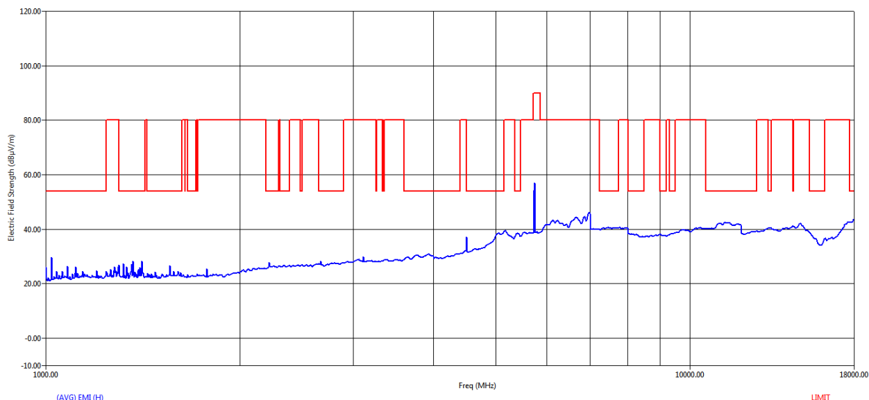
Figure 117 RE Graph from 1 GHz to 18 GHz using Average Detector – Horizontal Polarization
