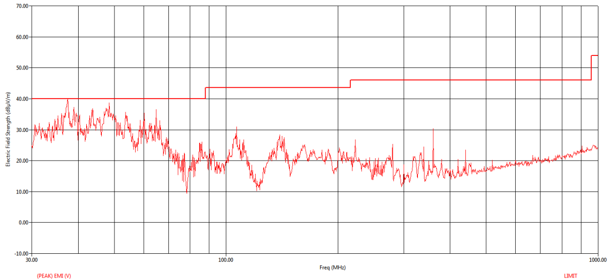
Figure 32 RE Graph from 30 MHz to 1 GHz using Peak detector – Vertical Polarization
