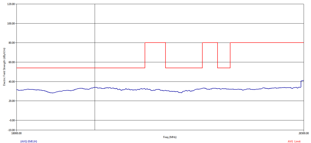
Figure 83 RE Graph from 18 GHz to 26.5 GHz using Average Detector – Horizontal Polarization
