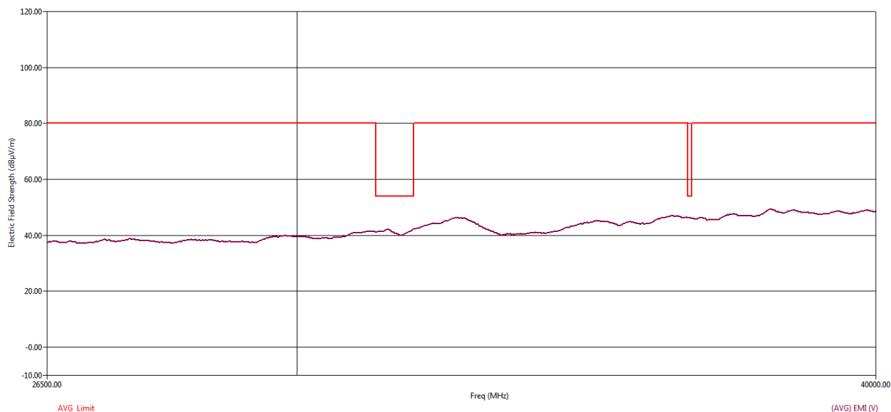
Figure 134 RE Graph from 26.5 GHz to 40 GHz using Average Detector – Vertical Polarization
