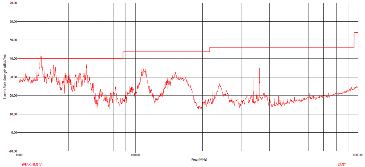
Figure 128 RE Graph from 30 MHz to 1 GHz using Peak Detector – Vertical Polarization
