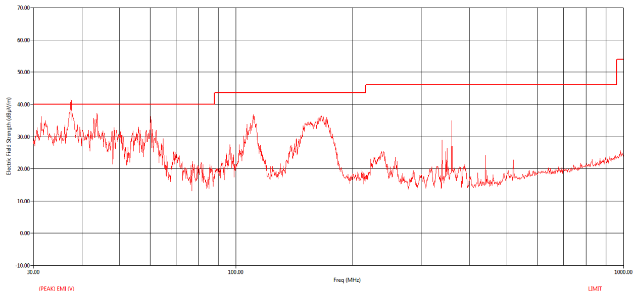
Figure 92 RE Graph from 30 MHz to 1 GHz using Peak Detector – Vertical Polarization
