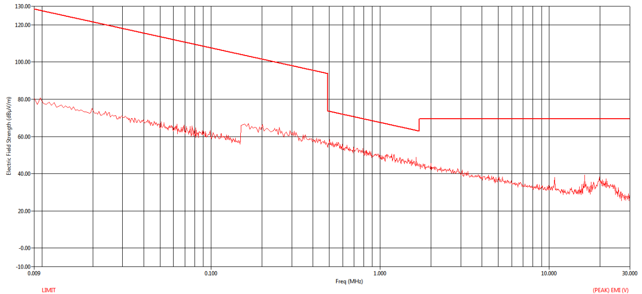
Figure 89 RE Graph from 9 kHz to 30 MHz using Peak Detector – Perpendicular
