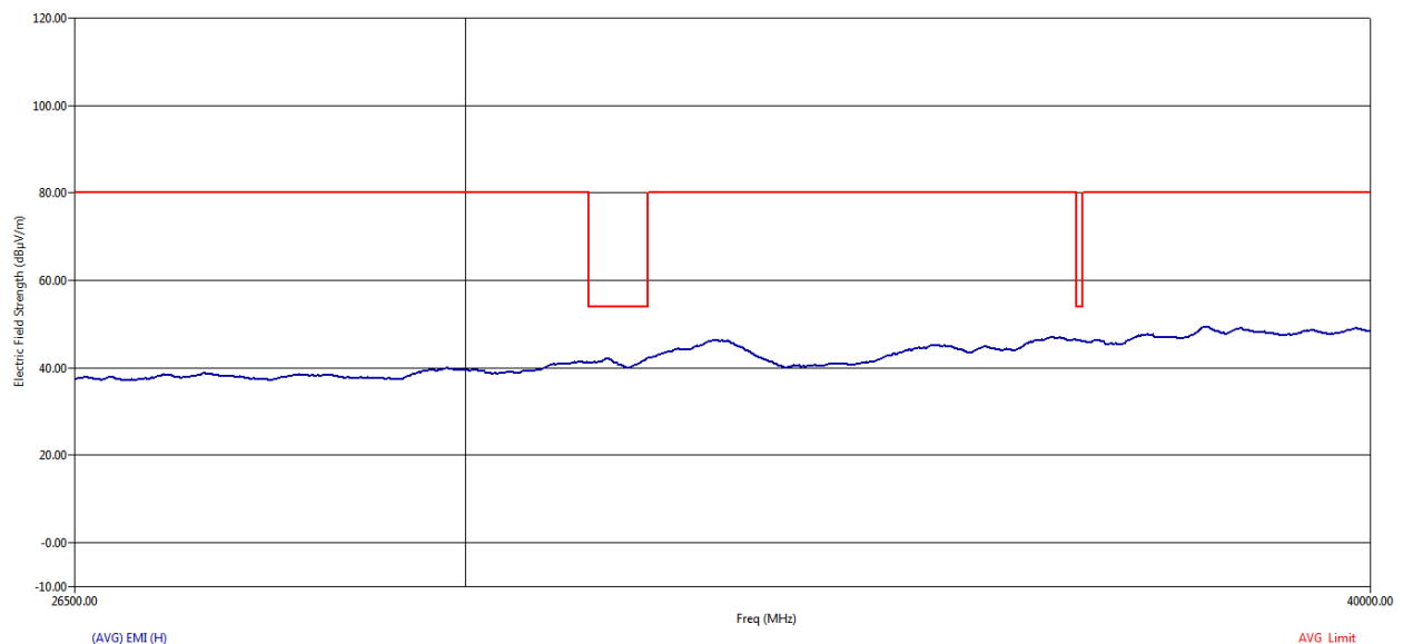
Figure 145 RE Graph from 26.5 GHz to 40 GHz using Average Detector – Horizontal Polarization
