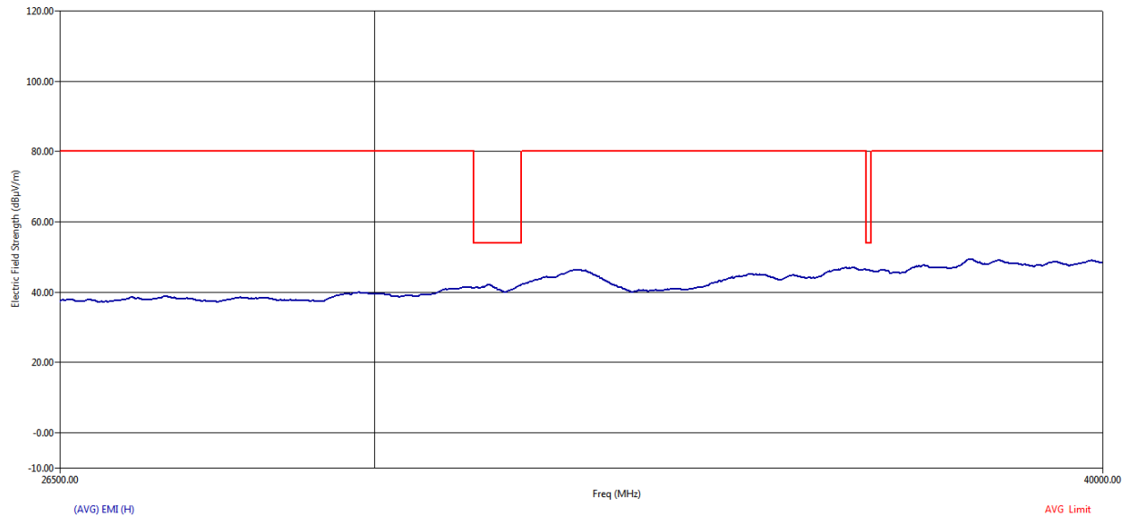
Figure 61 RE Graph from 26.5 GHz to 40 GHz using Average detector – Horizontal Polarization
