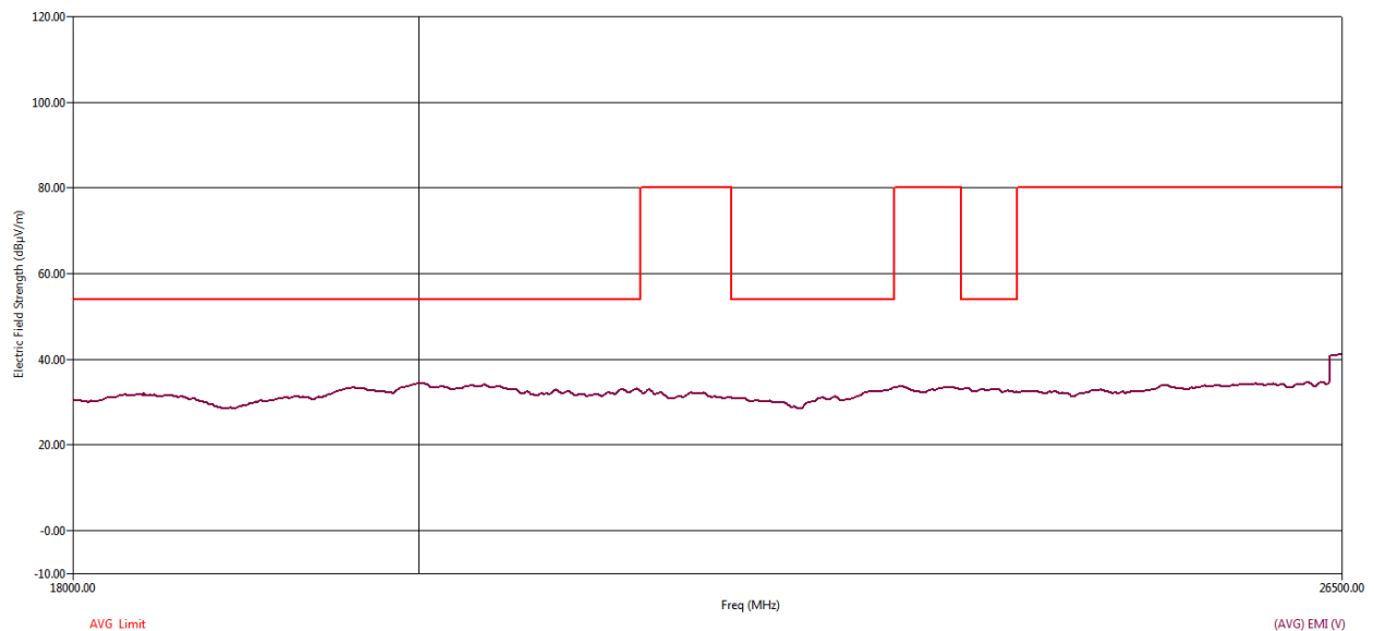
Figure 108 RE Graph from 18 GHz to 26.5 GHz using Average Detector – Vertical Polarization
