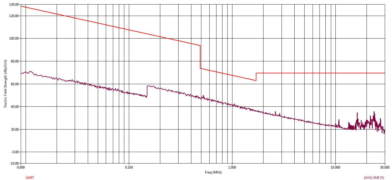
Figure 54 RE Graph from 9 kHz to 30 MHz using Average Detector – Perpendicular
