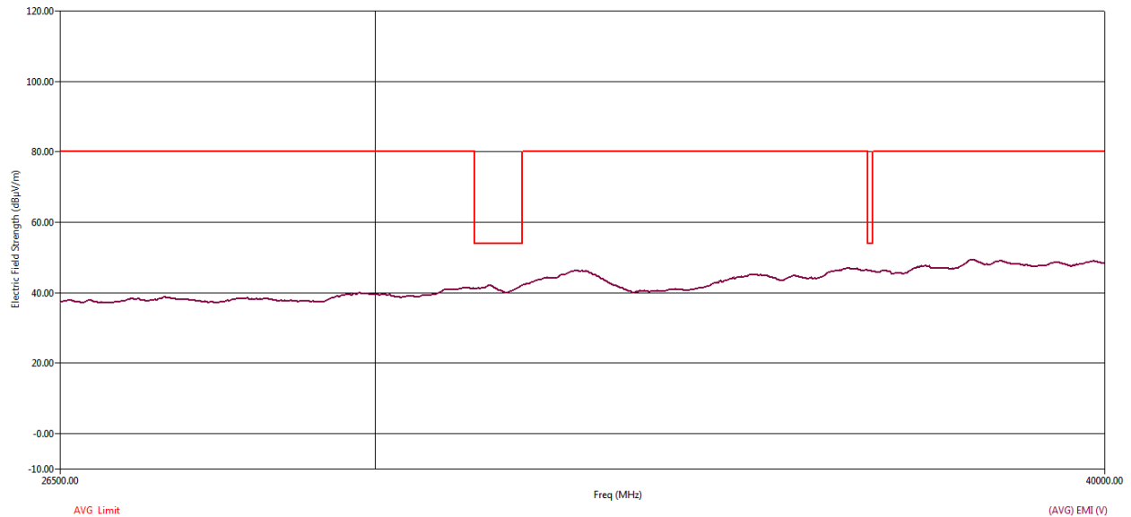
Figure 146 RE Graph from 26.5 GHz to 40 GHz using Average Detector – Vertical Polarization
