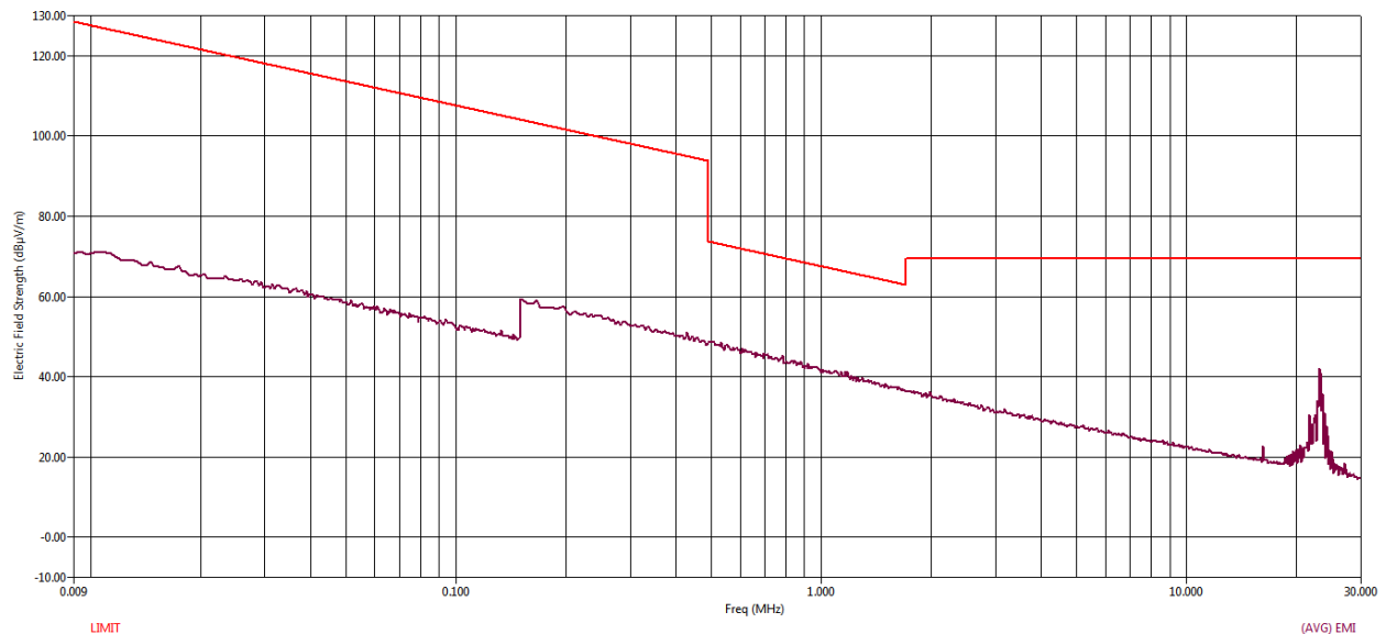
Figure 40 RE Graph from 9 kHz to 30 MHz using Average Detector – Parallel
