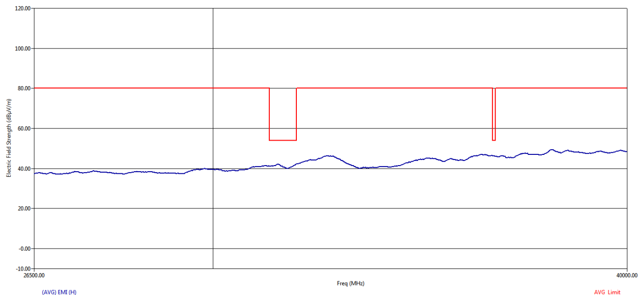
Figure 73 RE Graph from 26.5 GHz to 40 GHz using Average detector – Horizontal Polarization
