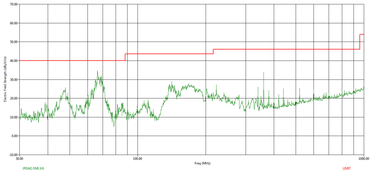
Figure 19 RE Graph from 30 MHz to 1 GHz using Peak Detector – Horizontal Polarization
