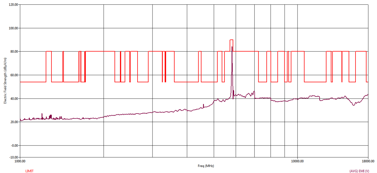
Figure 106 RE Graph from 1 GHz to 18 GHz using Average Detector – Vertical Polarization
