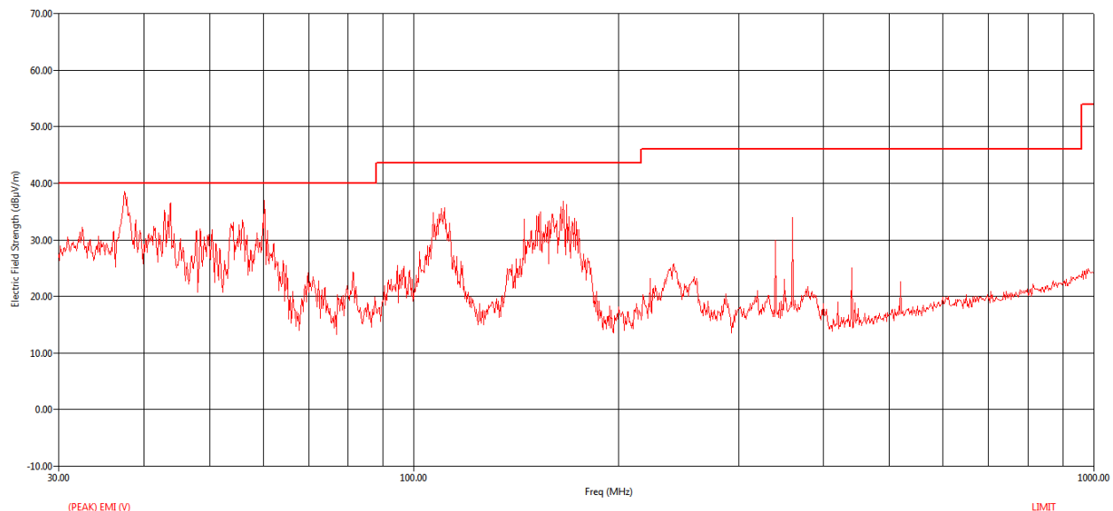
Figure 140 RE Graph from 30 MHz to 1 GHz using Peak Detector – Vertical Polarization
