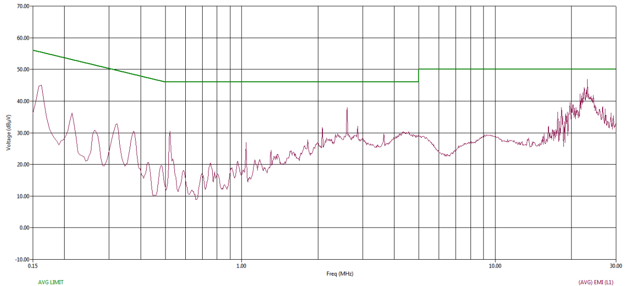
Figure 195 CE graph from 150 kHz to 30 MHz using Average detector – Line
