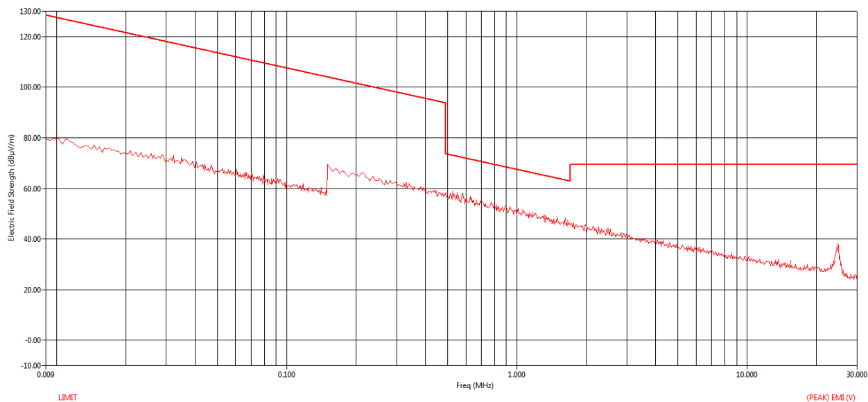
Figure 135 RE Graph from 9 kHz to 30 MHz using Peak Detector – Parallel
