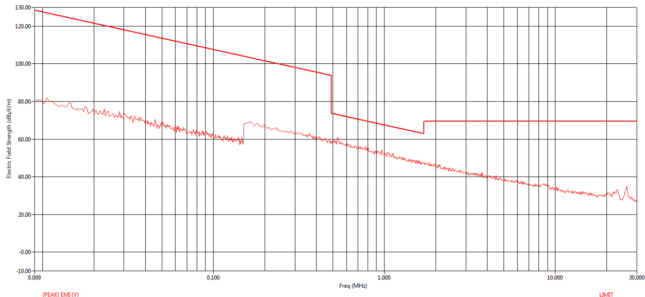
Figure 41: 10 MHz, 17 dBi, Low channel: Peak RE graph - 9 kHz to 30 MHz - Perpendicular
