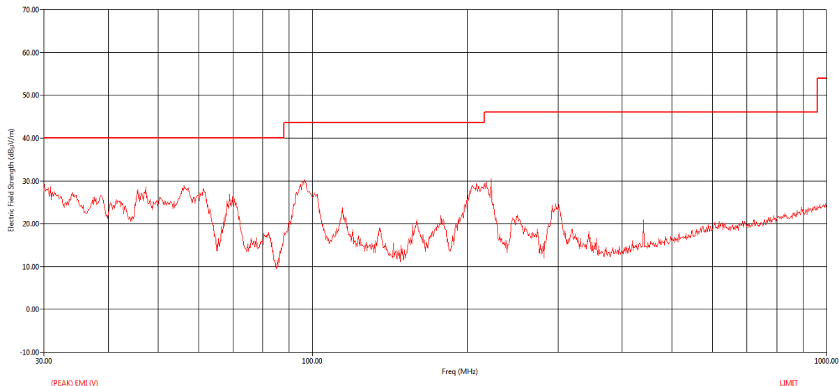
Figure 8: 40 MHz, 17 dBi, Low channel: Peak RE graph - 30 MHz to 1 GHz - Vertical
