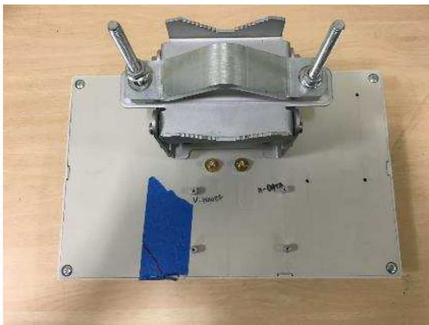
Figure 5: Photograph of 17 dBi Receive Antenna
