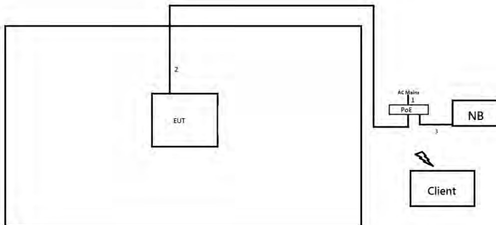
Test Setup Diagram - Radiated Test <Beamforming>
