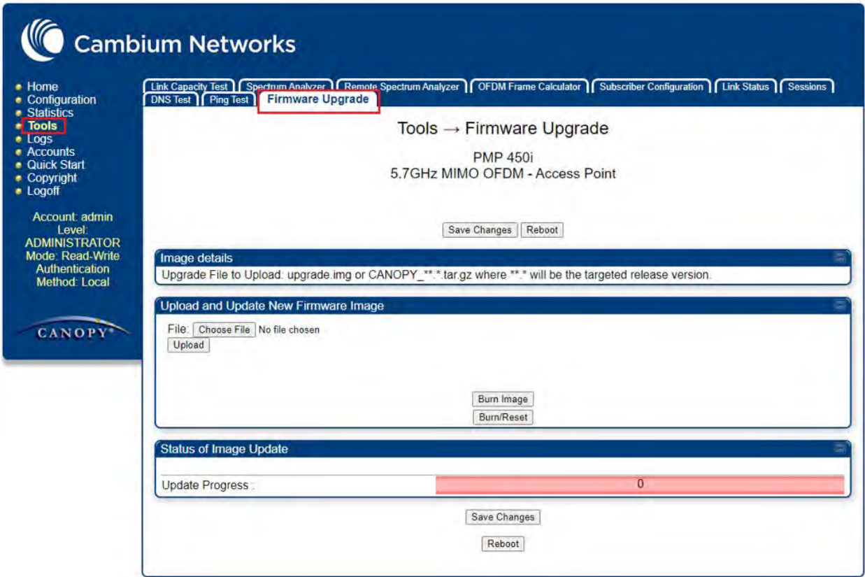
Figure 107: Firmware upgrade
