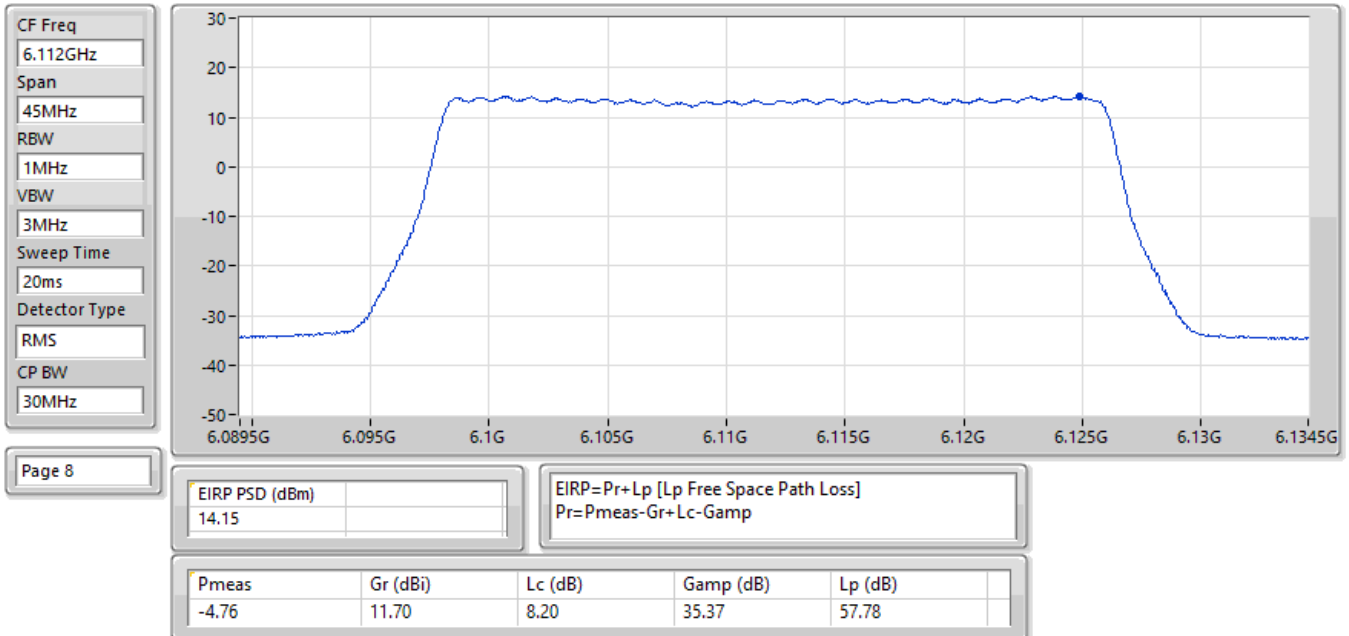
EIRP PSD; Band: 6.2G; QPSK; BWch: 30MHz; Nss: 1; Nant: 2; Ch: 6112MHz; TX
