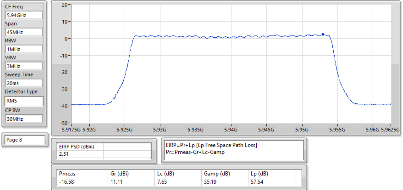
EIRP PSD; Band: 6.2G; QPSK; BWch: 30MHz; Nss: 1; Nant: 2; Ch: 5940MHz; TX
