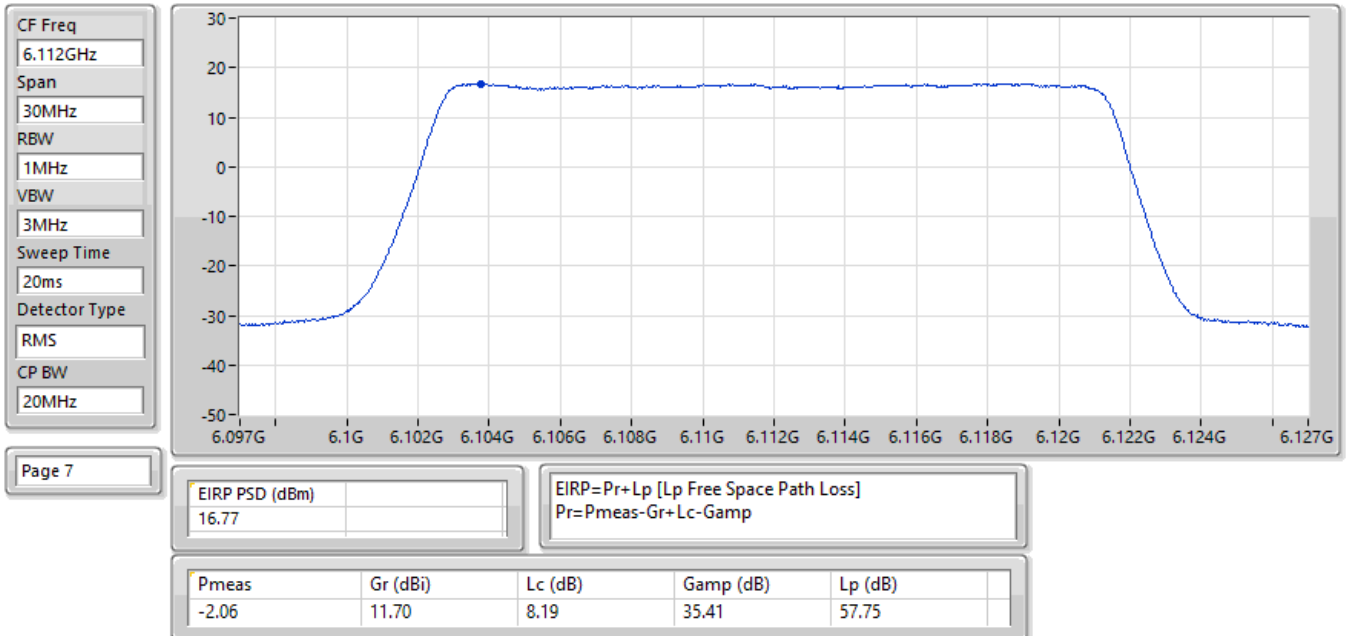
EIRP PSD; Band: 6.2G; QPSK; BWch: 20MHz; Nss: 1; Nant: 2; Ch: 6112MHz; TX
