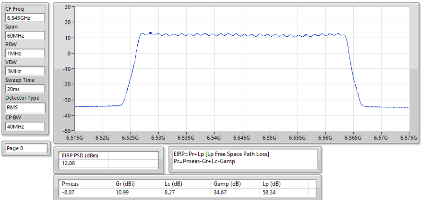
EIRP PSD; Band: 6.7G; QPSK; BWch: 40MHz; Nss: 1; Nant: 2; Ch: 6545MHz; TX
