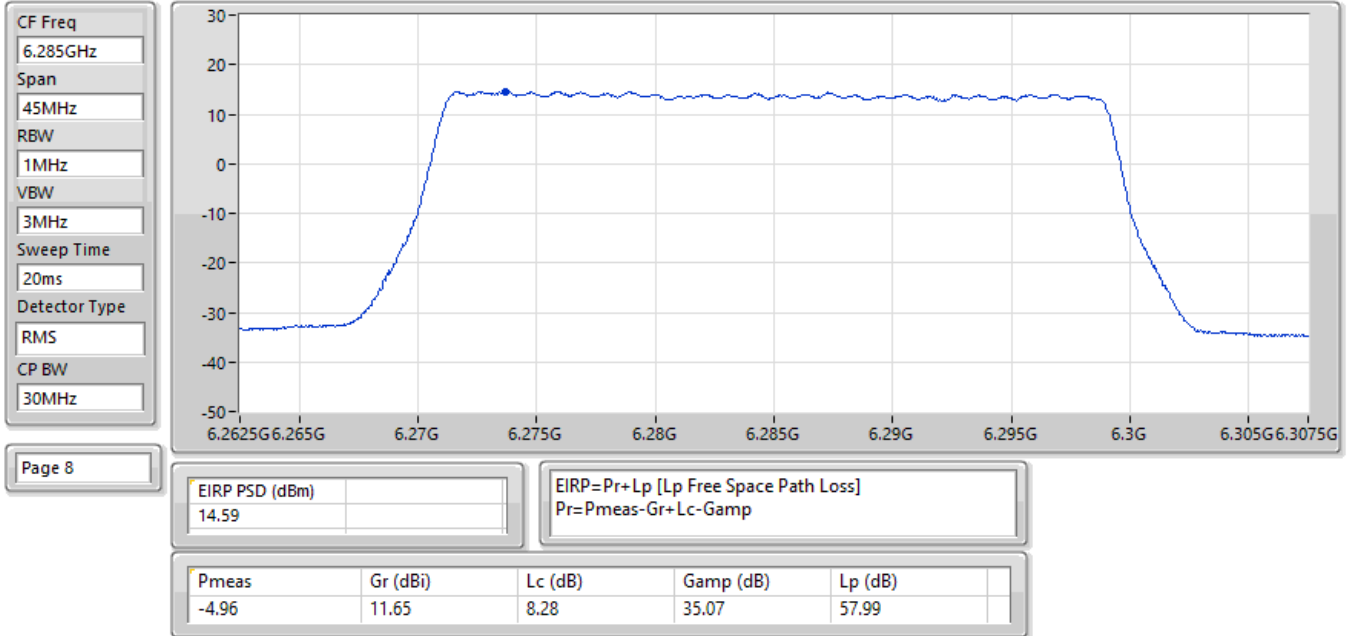
EIRP PSD; Band: 6.2G; QPSK; BWch: 30MHz; Nss: 1; Nant: 2; Ch: 6285MHz; TX
