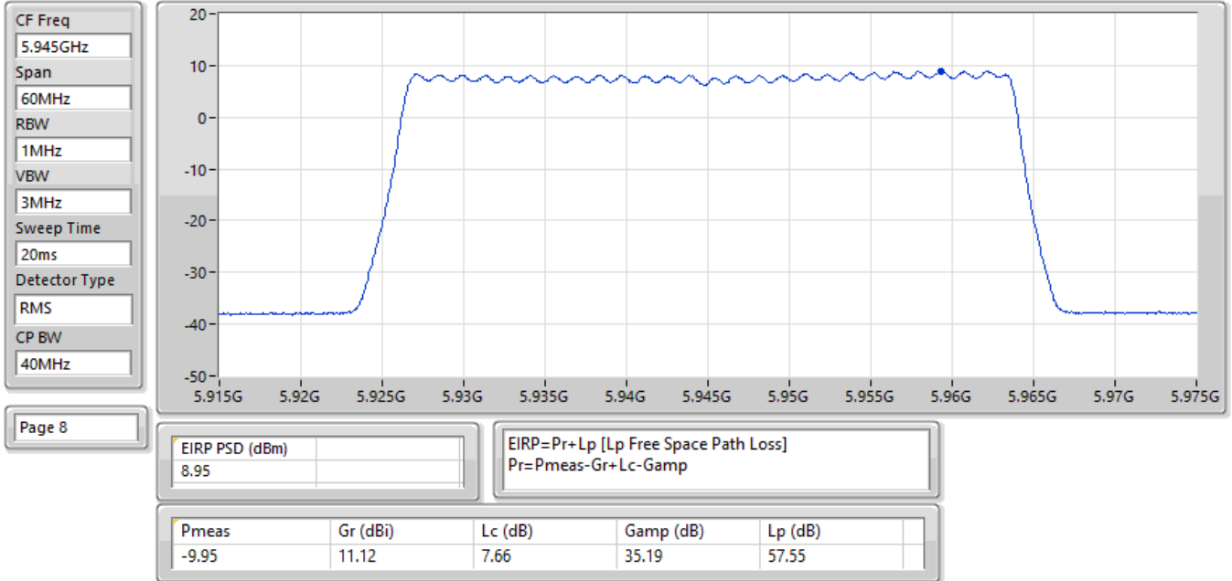
EIRP PSD; Band: 6.2G; QPSK; BWch: 40MHz; Nss: 1; Nant: 2; Ch: 5945MHz; TX
