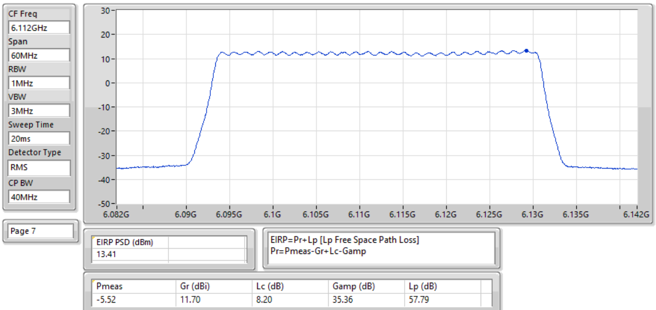
EIRP PSD; Band: 6.2G; QPSK; BWch: 40MHz; Nss: 1; Nant: 2; Ch: 6112MHz; TX
