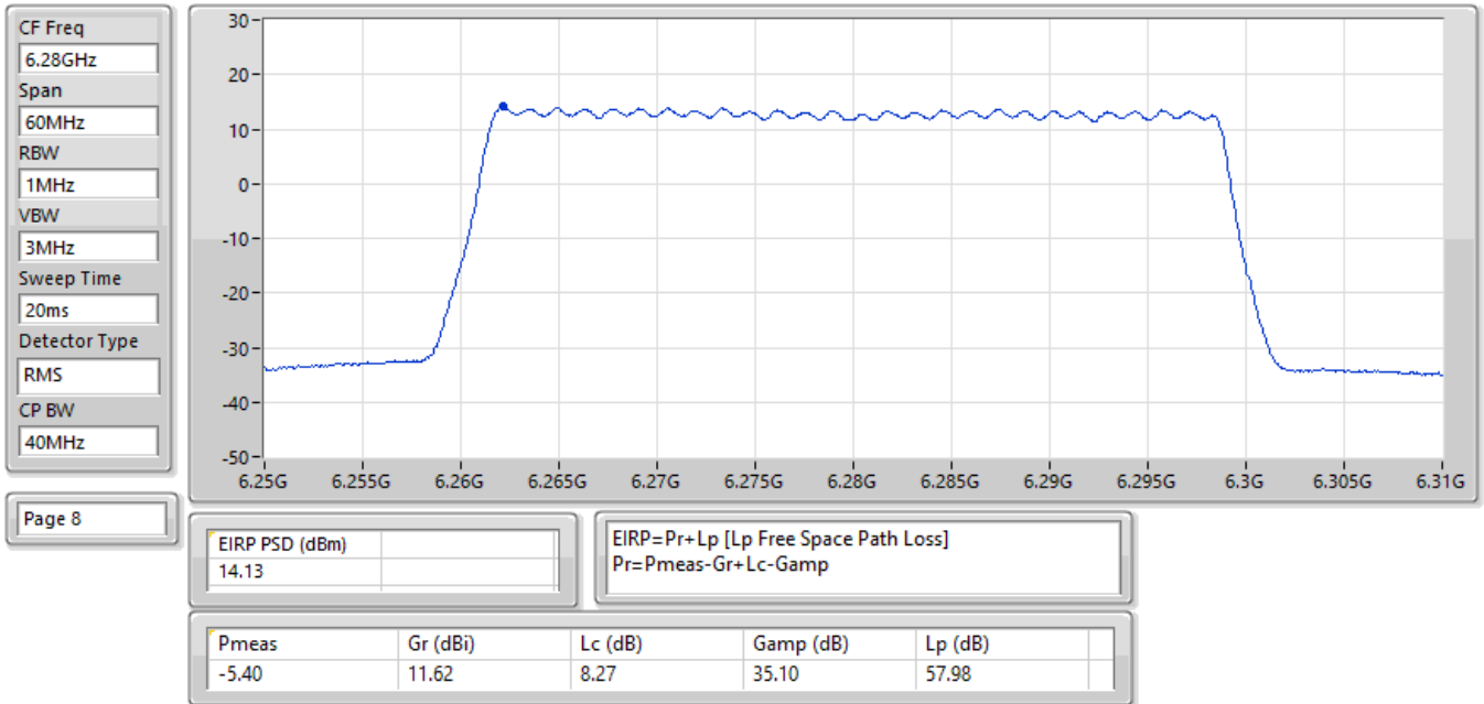
EIRP PSD; Band: 6.2G; QPSK; BWch: 40MHz; Nss: 1; Nant: 2; Ch: 6280MHz; TX
