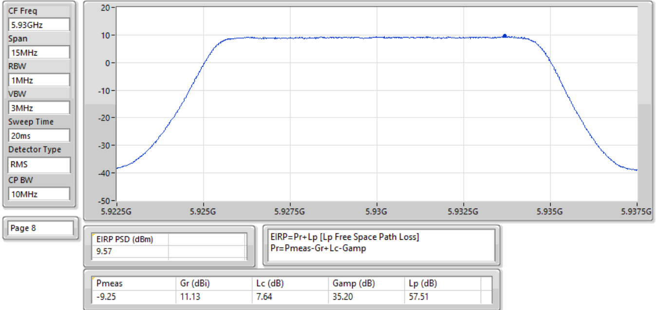
EIRP PSD; Band: 6.2G; QPSK; BWch: 10MHz; Nss: 1; Nant: 2; Ch: 5930MHz; TX
