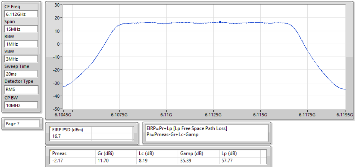
EIRP PSD; Band: 6.2G; QPSK; BWch: 10MHz; Nss: 1; Nant: 2; Ch: 6112MHz; TX
