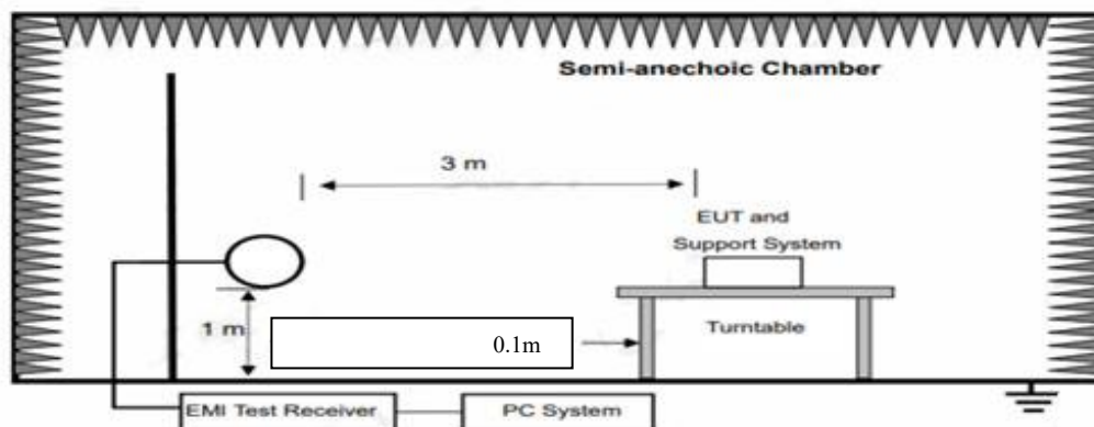
Test set-up of radiated disturbance (Below 30MHz)
