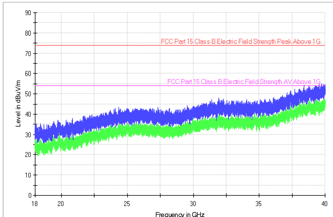
Electric Field Strength 18-40 GdBuV
