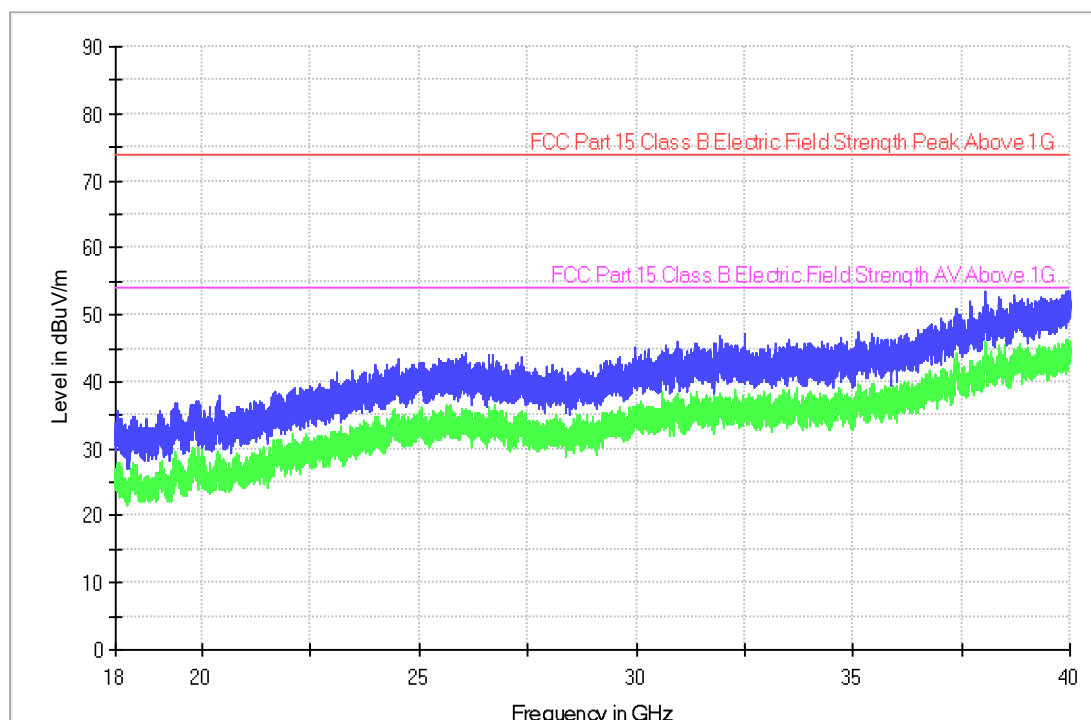
Electric Field Strength 18-40 GdBuV
