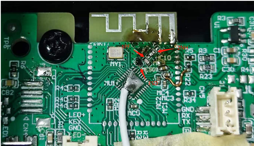
Antenna position
