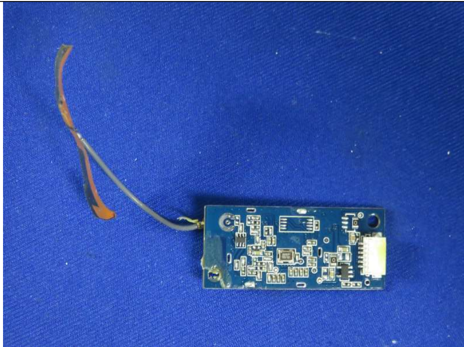
12. Figure PCB of the RF board-Back View
