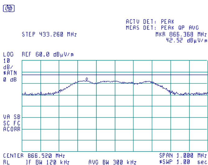
Plot 7.2.28 Radiated emission measurements at the second harmonic frequency, UHF2 transmitter
