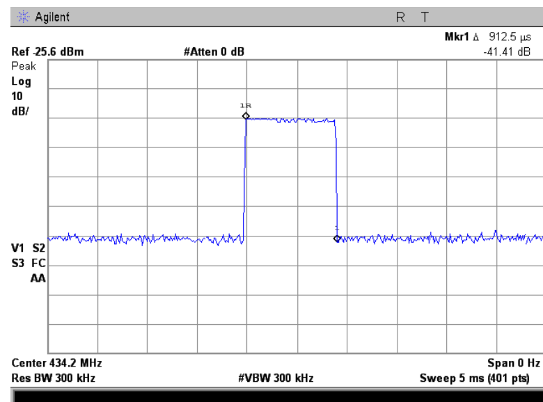
Plot 7.2.64 Transmission pulse duration at 434.2 MHz
