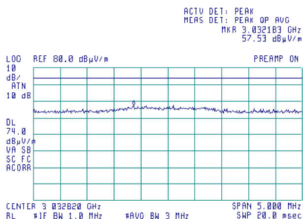
Plot 7.2.40 Radiated emission measurements at the seventh harmonic frequency, UHF2 transmitter
