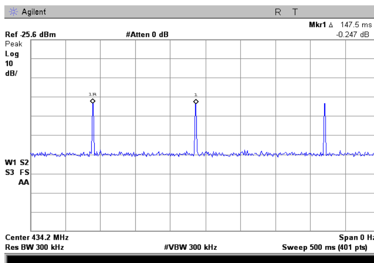
Plot 7.1.6 Transmission duration at port UHF2, 434.2 MHz
