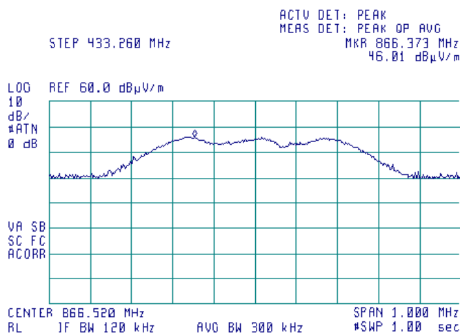
Plot 7.2.30 Radiated emission measurements at the second harmonic frequency, UHF3 transmitter
