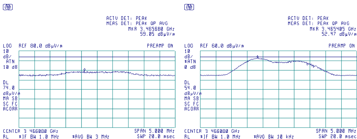
Plot 7.2.58 Radiated emission measurements at the eighth harmonic frequency, UHF3 transmitter
