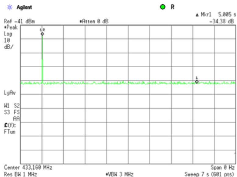
Plot 7.1.1 Transmitter shut down test result at port UHF2, 433.2 MHz
