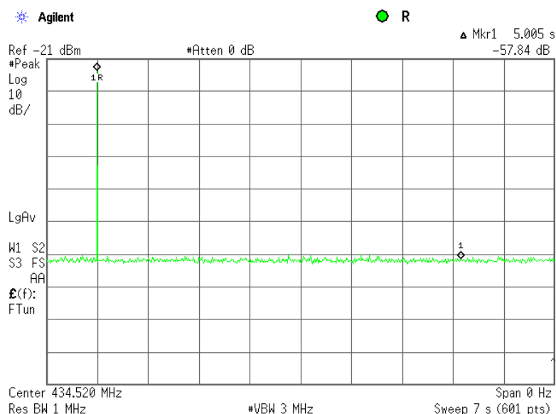
Plot 7.1.7 Transmitter shut down test result at port UHF3
