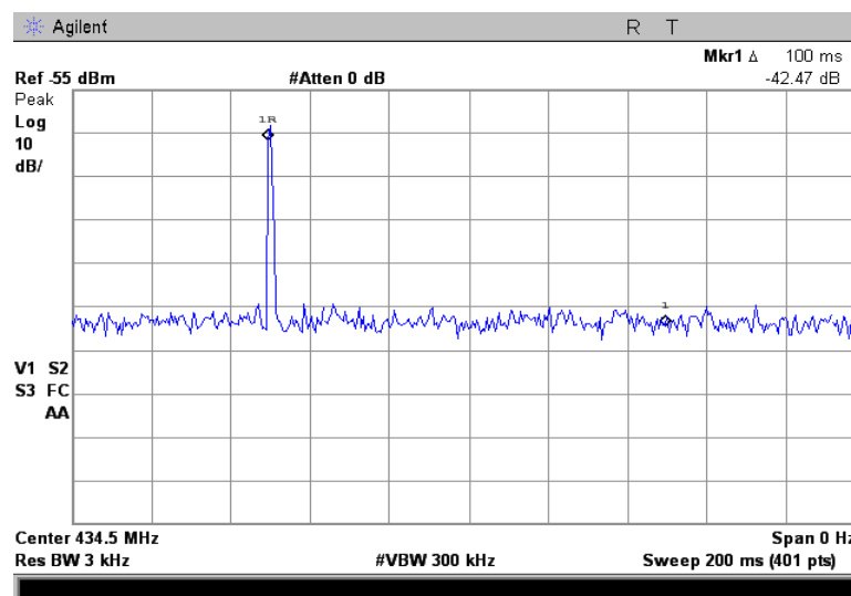
Plot 7.1.8 Transmission duration at port UHF3
