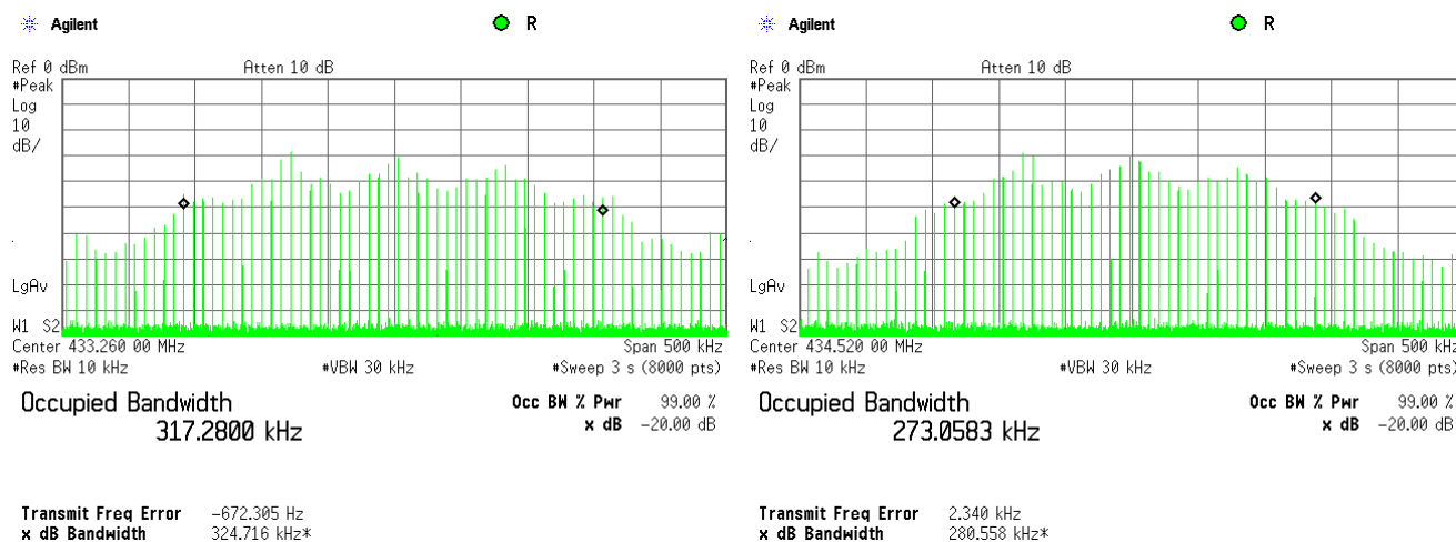
Plot 7.3.3 Occupied bandwidth test result Antenna 3
