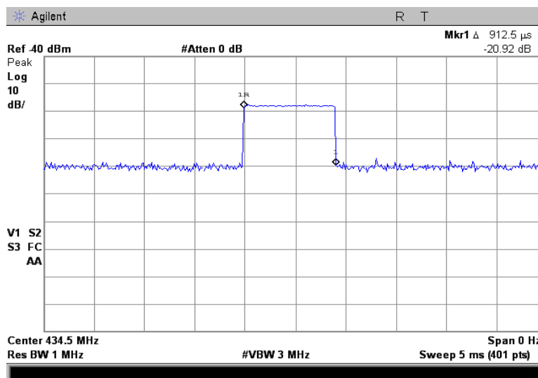
Plot 7.1.9 Pulse duration at port UHF3
