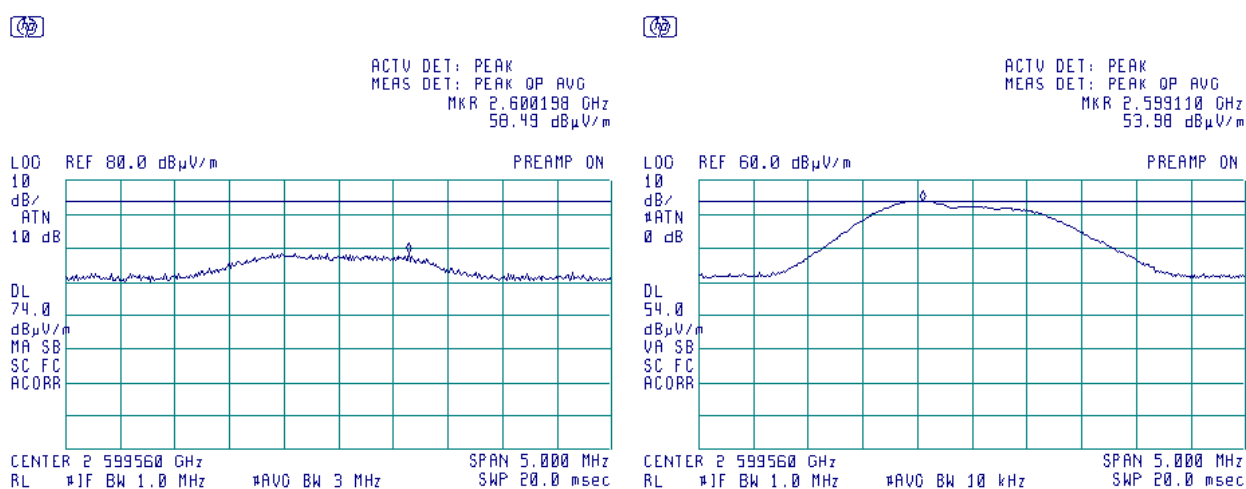
Plot 7.2.38 Radiated emission measurements at the sixth harmonic frequency, UHF2 transmitter
