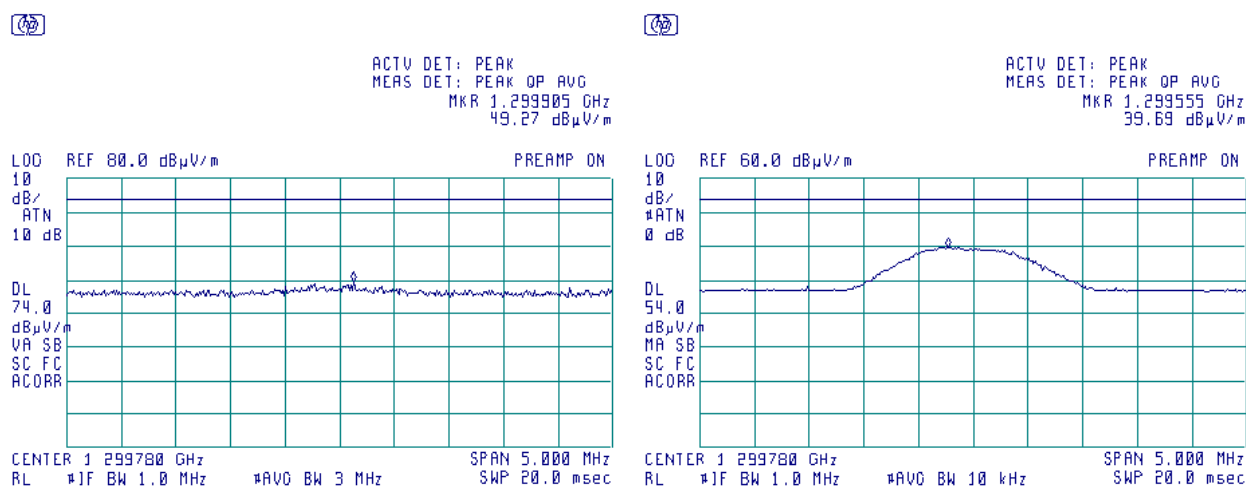
Plot 7.2.32 Radiated emission measurements at the third harmonic frequency, UHF2 transmitter
