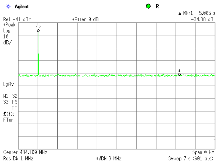
Plot 7.1.2 Transmitter shut down test result at port UHF2, 434.2 MHz
