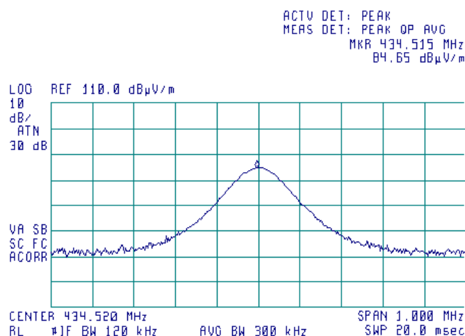
Plot 7.2.6 Radiated emission measurements at the fundamental frequency 434.52 MHz, UHF2 transmitter
