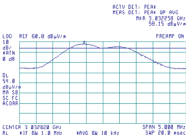
Plot 7.2.56 Radiated emission measurements at the seventh harmonic frequency, UHF3 transmitter
