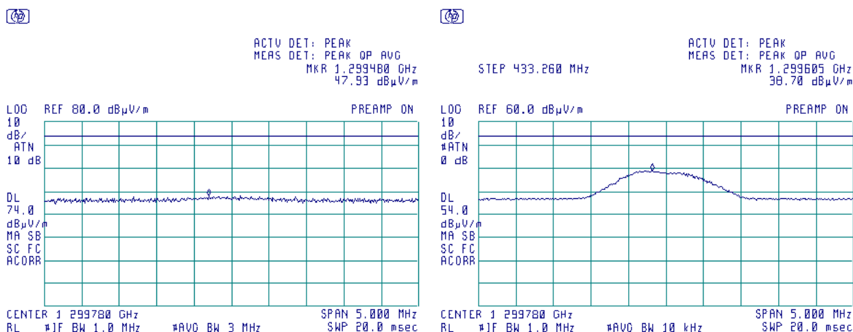
Plot 7.2.48 Radiated emission measurements at the third harmonic frequency, UHF3 transmitter
