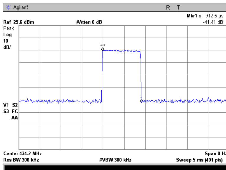
Plot 7.1.4 Pulse duration at port UHF2, 434.2 MHz
