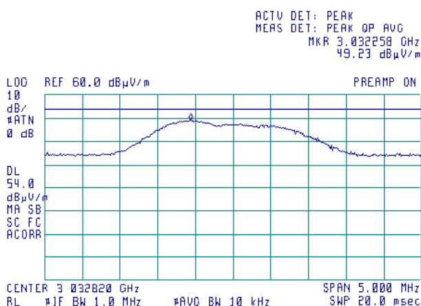
Plot 7.2.40 Radiated emission measurements at the seventh harmonic frequency, UHF2 transmitter
