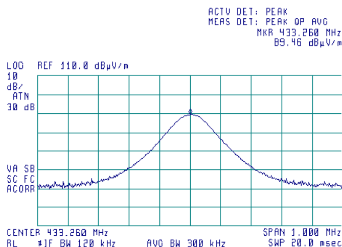
Plot 7.2.12 Radiated emission measurements at the fundamental frequency 433.26 MHz, UHF3 transmitter
