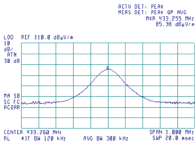
Plot 7.2.2 Radiated emission measurements at the fundamental frequency 433.26 MHz, UHF2 transmitter t
