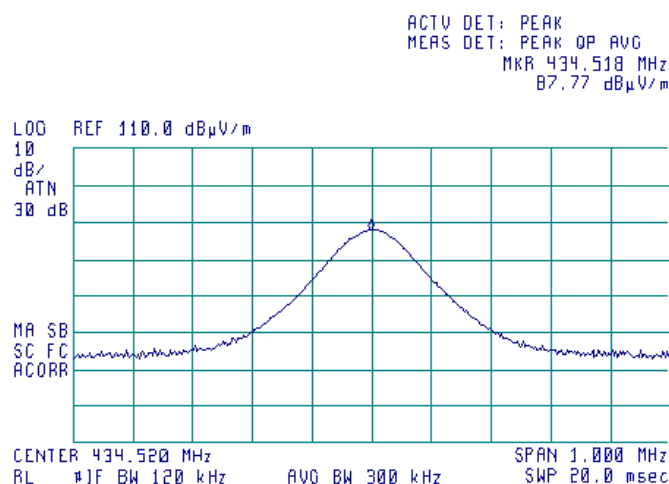
Plot 7.2.8 Radiated emission measurements at the fundamental frequency 434.52 MHz, UHF2 transmitter
