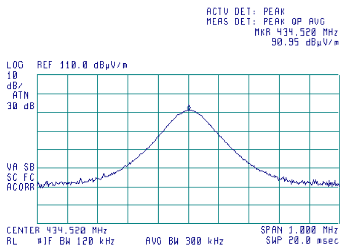
Plot 7.2.16 Radiated emission measurements at the fundamental frequency 434.52 MHz, UHF3 transmitter
