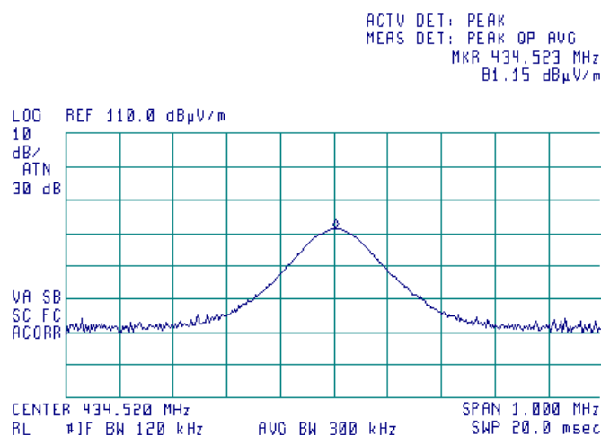
Plot 7.2.14 Radiated emission measurements at the fundamental frequency 434.52 MHz, UHF3 transmitter
