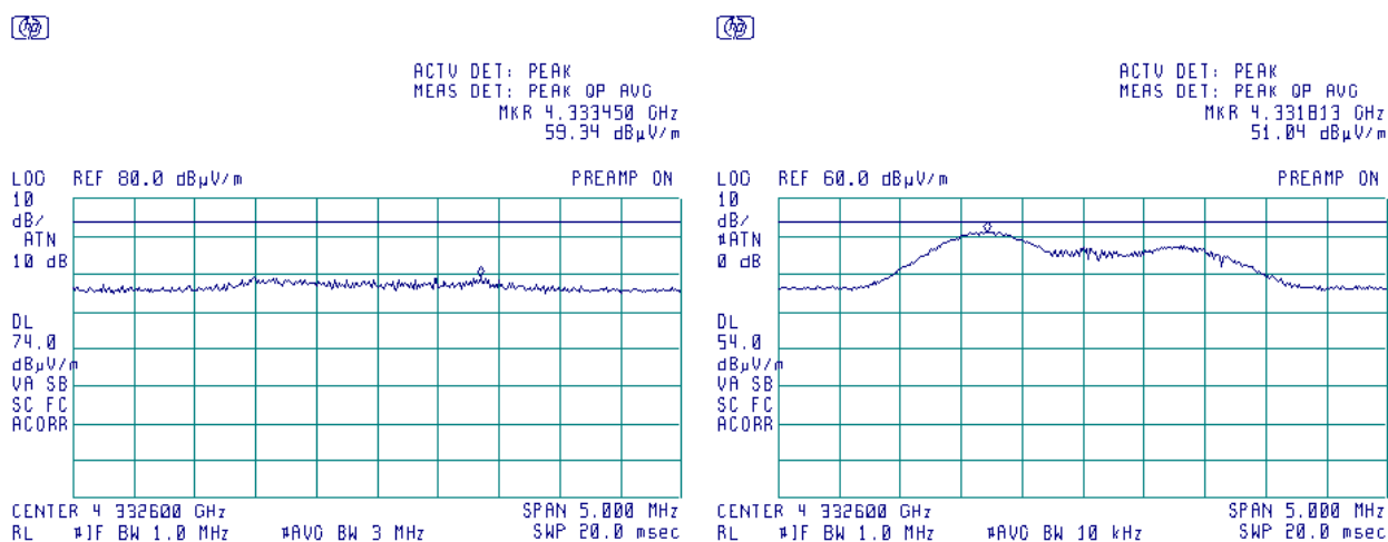
Plot 7.2.62 Radiated emission measurements at the tenth harmonic frequency, UHF3 transmitter
