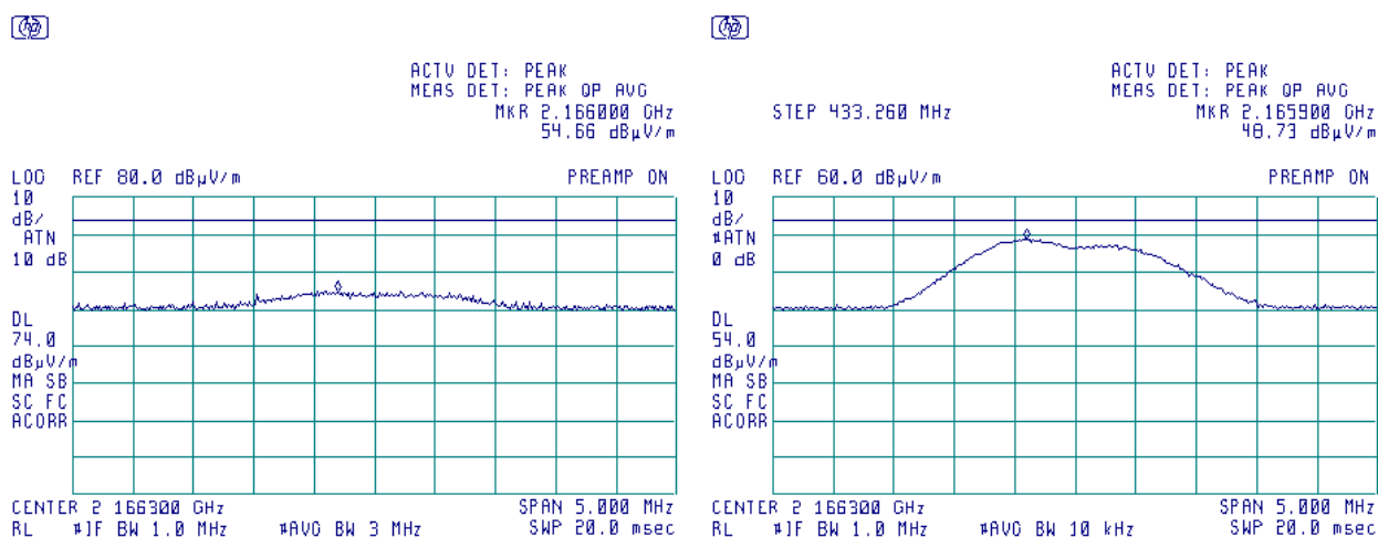
Plot 7.2.52 Radiated emission measurements at the fifth harmonic frequency, UHF3 transmitter
