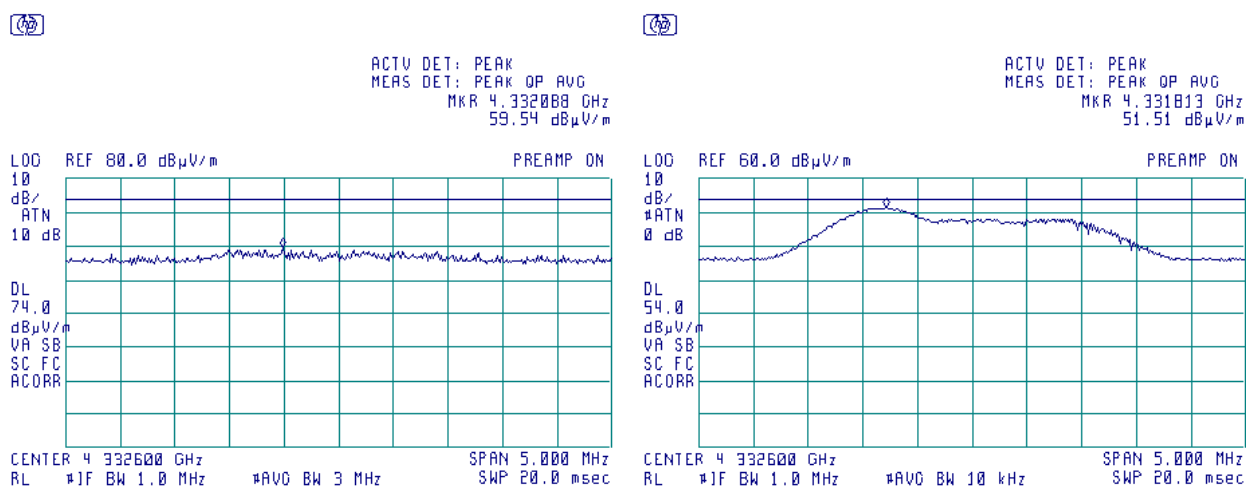
Plot 7.2.46 Radiated emission measurements at the tenth harmonic frequency, UHF2 transmitter
