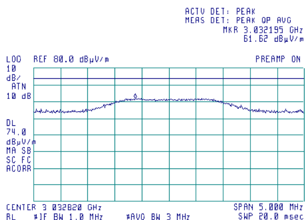
Plot 7.2.56 Radiated emission measurements at the seventh harmonic frequency, UHF3 transmitter
