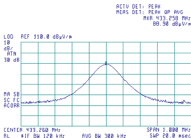
Plot 7.2.4 Radiated emission measurements at the fundamental frequency 433.26 MHz, UHF2 transmitter
