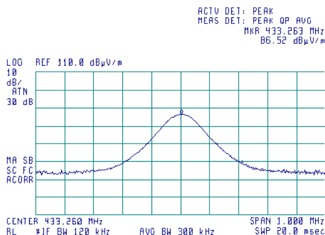
Plot 7.2.10 Radiated emission measurements at the fundamental frequency 433.26 MHz, UHF3 transmitter
