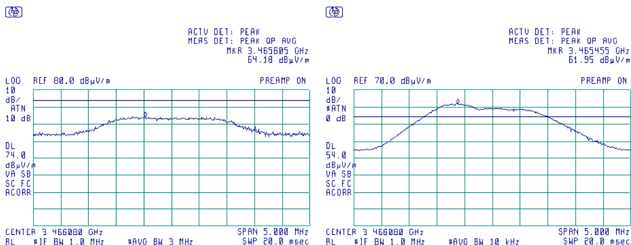
Plot 7.2.42 Radiated emission measurements at the eighth harmonic frequency, UHF2 transmitter
