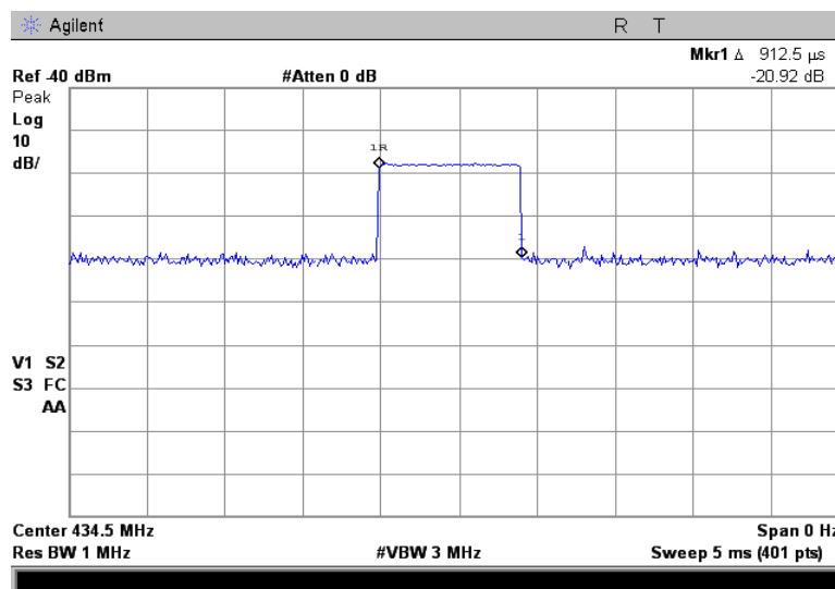
Plot 7.2.65 Transmission pulse duration at 434.52 MHz
