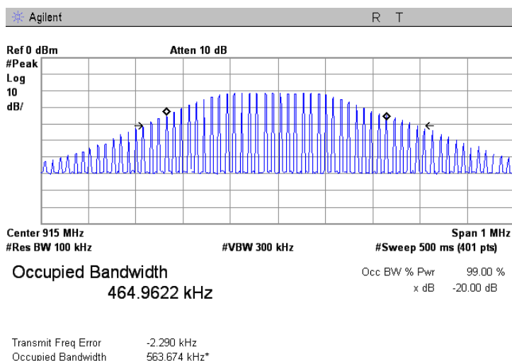
Plot 7.5.4 Occupied bandwidth test result at mid frequency
