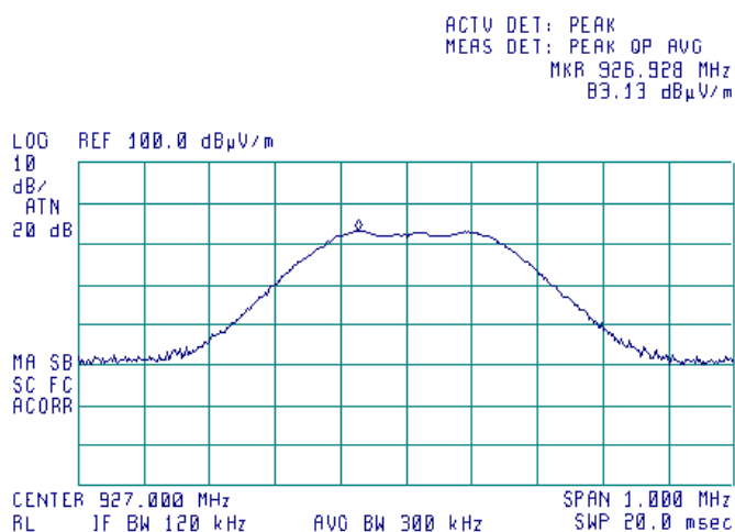
Plot 7.1.10 Radiated emission measurements at the high fundamental frequency
