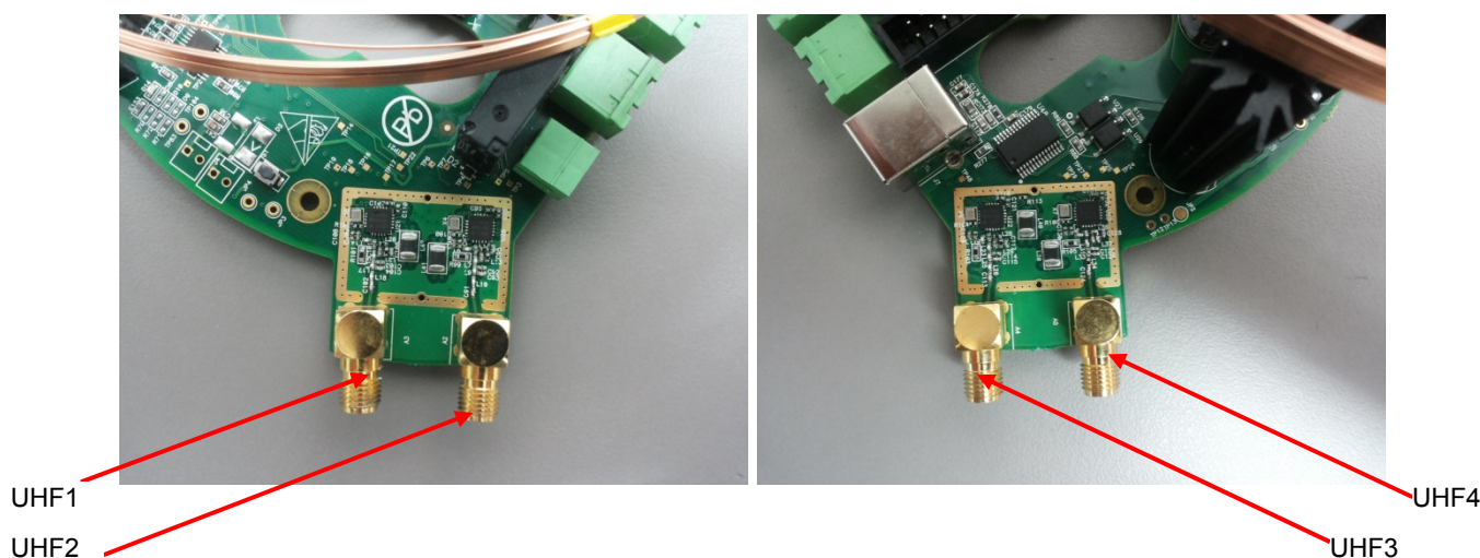
Photograph 7.4.1 Antenna assembly
