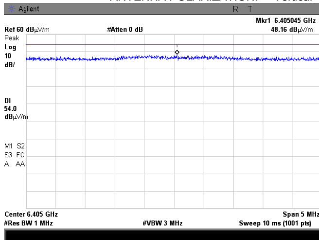
Plot 7.1.45 Radiated emission measurements at the seventh harmonic at mid frequency
