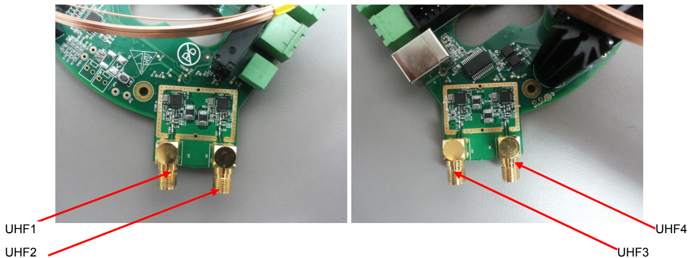
Photograph 7.6.1 Antenna assembly
