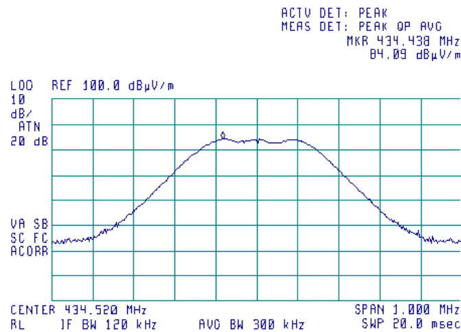
Plot 7.3.6 Radiated emission measurements at the fundamental frequency 434.52 MHz
