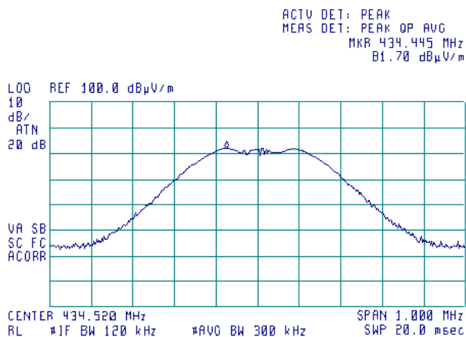
Plot 7.2.8 Radiated emission measurements at the fundamental frequency 434.52 MHz
