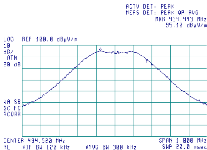
Plot 7.2.6 Radiated emission measurements at the fundamental frequency 434.52 MHz
