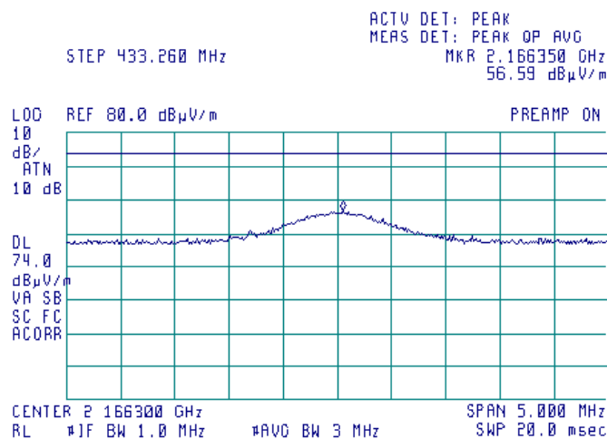
Plot 7.3.24 Radiated emission measurements at the fifth harmonic frequency
