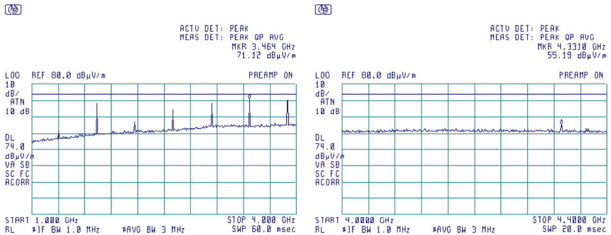
Plot 7.2.13 Radiated emission measurements from 1000 to 4400 MHz
