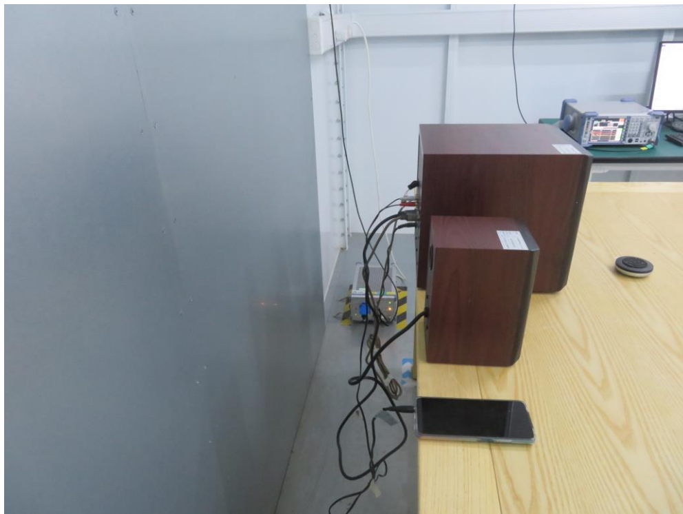
Description: Back View of AC Conducted Emission Test Setup
