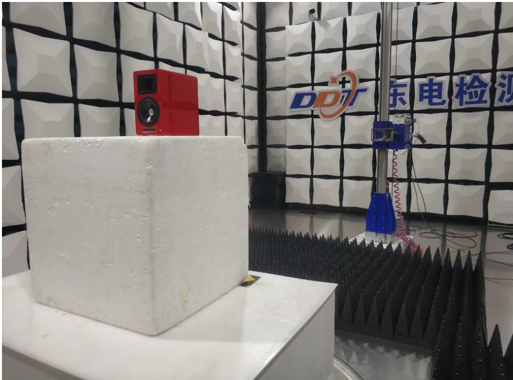
Photograph 3: Set-up for Radiated Spurious Emission, above 1GHz
