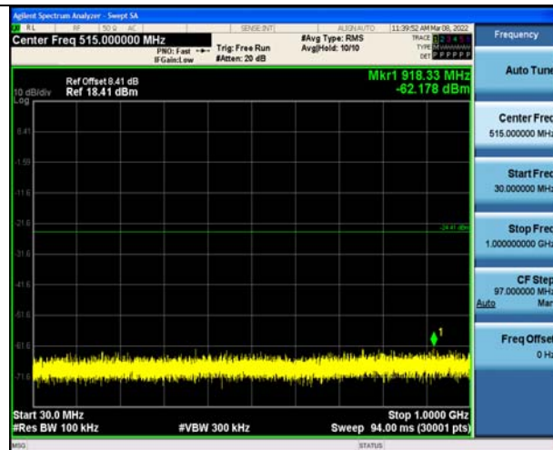
\pi/4 -DQPSK on Channel 39
