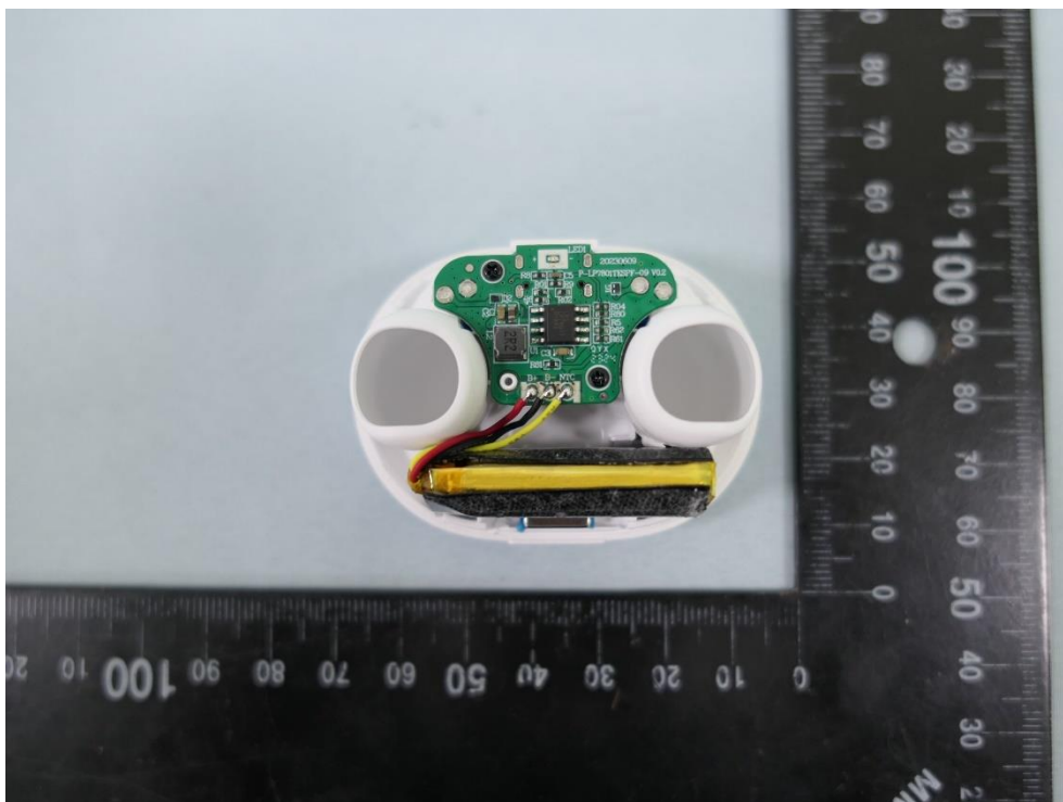
(24) EUT Photo_ Charging Box
