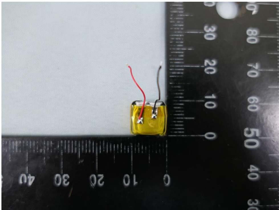
(16) EUT Photo_Right Ear (Battery: Golden CEL)
