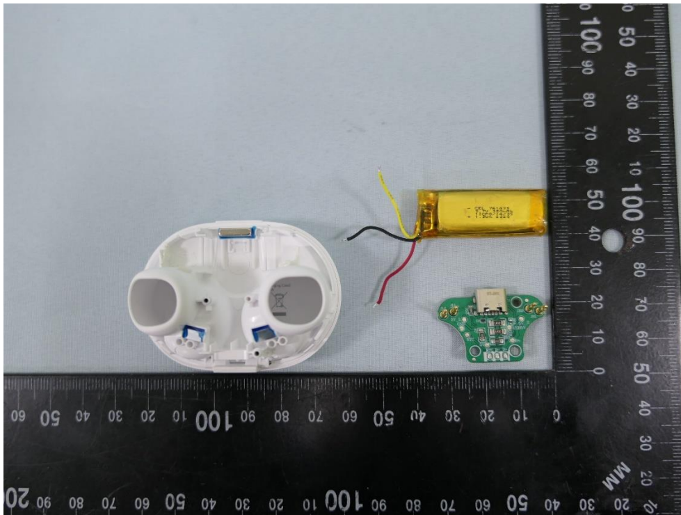
(25) EUT Photo_ Charging Box (Battery: Golden CEL)
