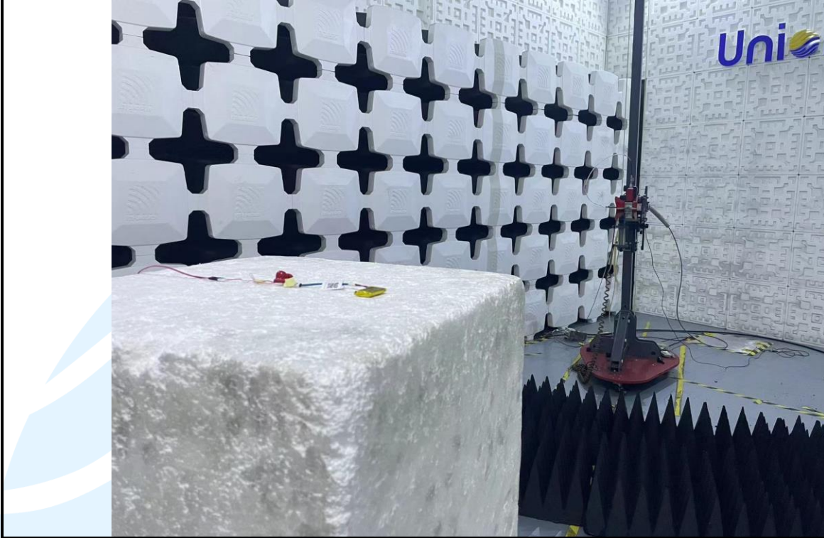
Radiated emission Test Setup (Above 1 GHz) _ Left Ear
