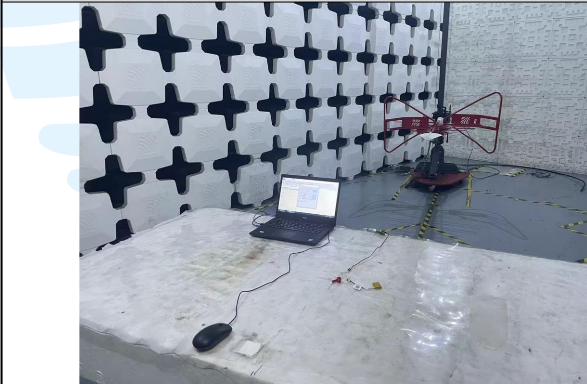
Radiated emission Test Setup (30 MHz~1 GHz)_ Right Ear
