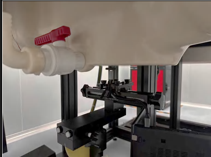
Tip of EUT with Dongle with 0 cm Gap
