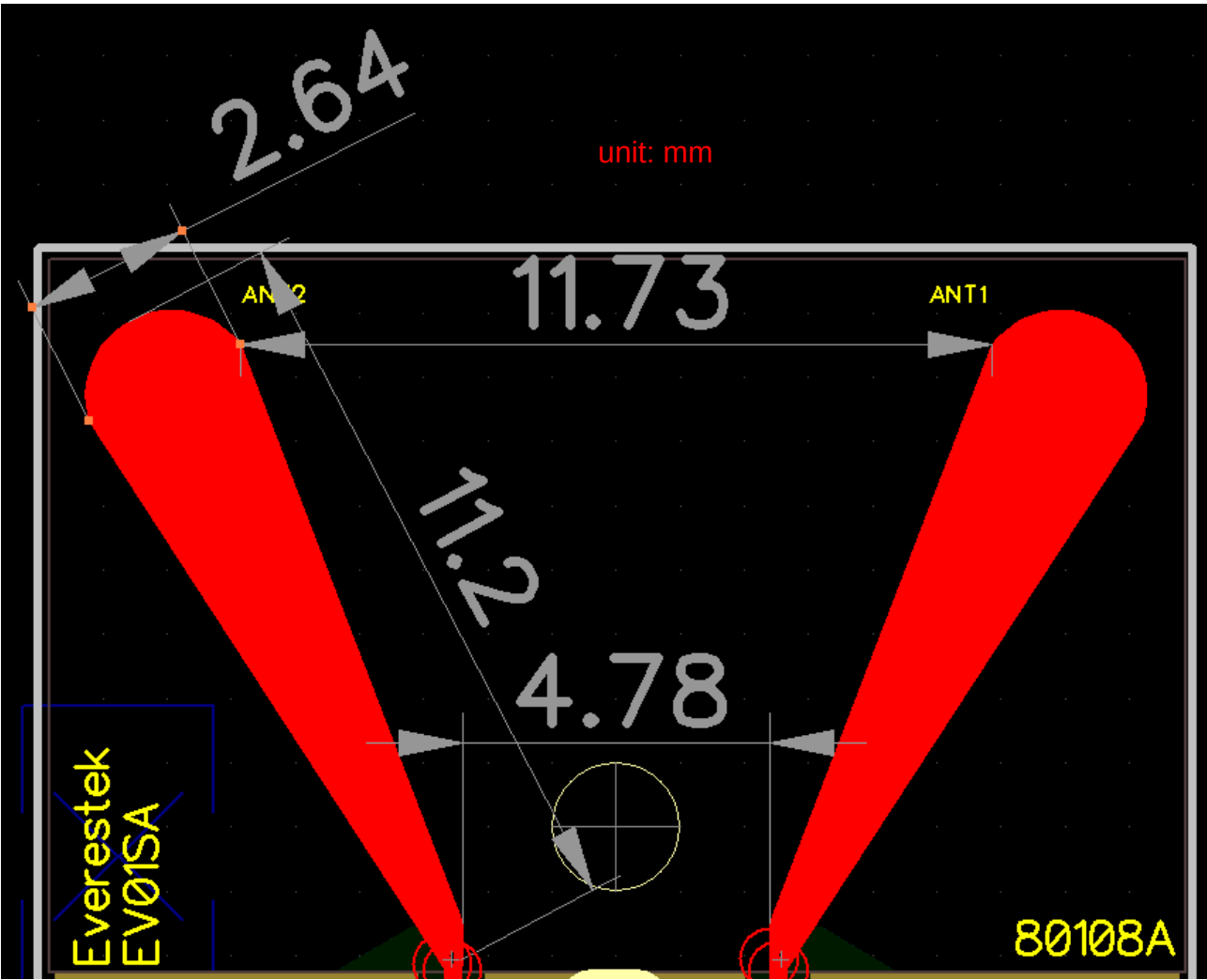
Picture of Antenna
