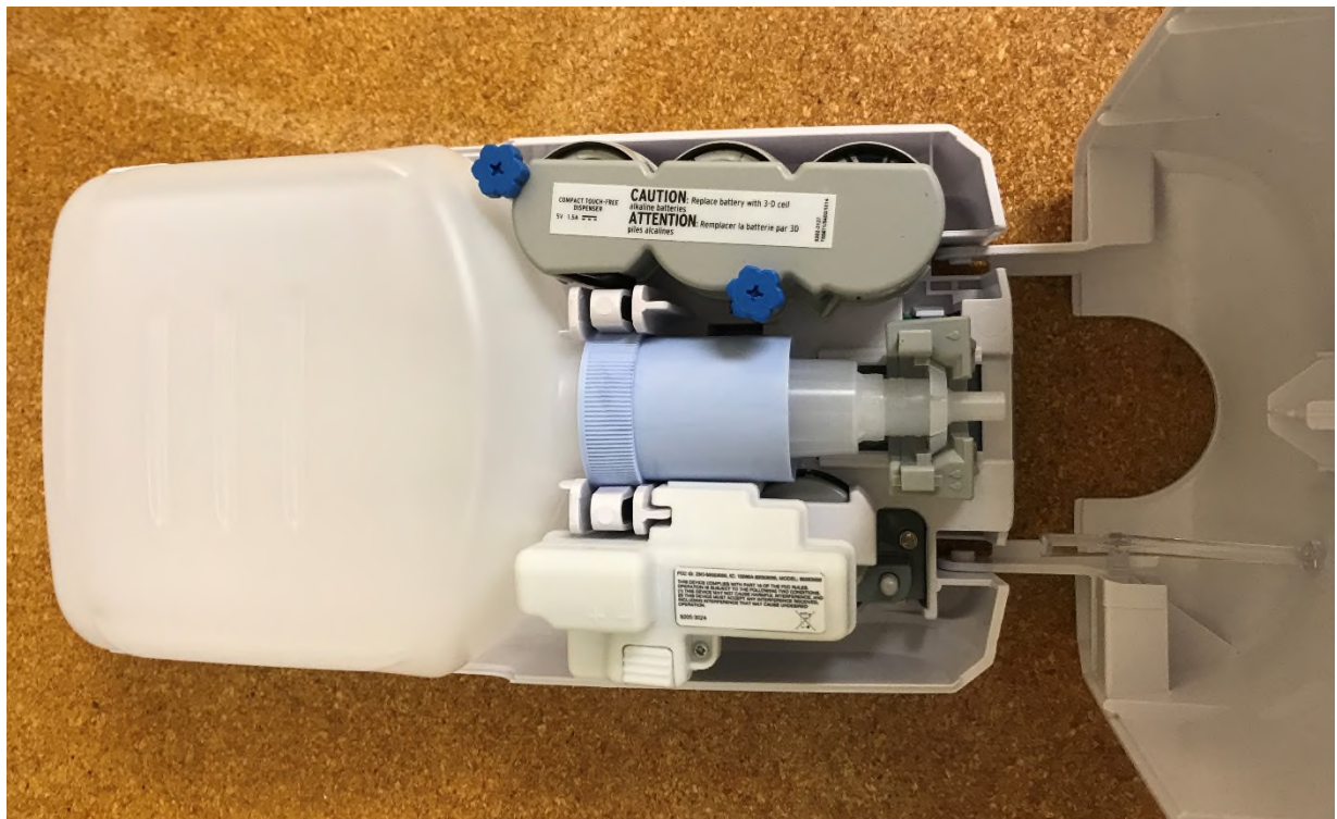
Figure 7: EUT Installed in Host
