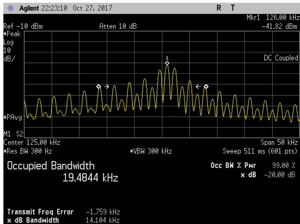
Figure 7.2.2-1: 20 dB BW
