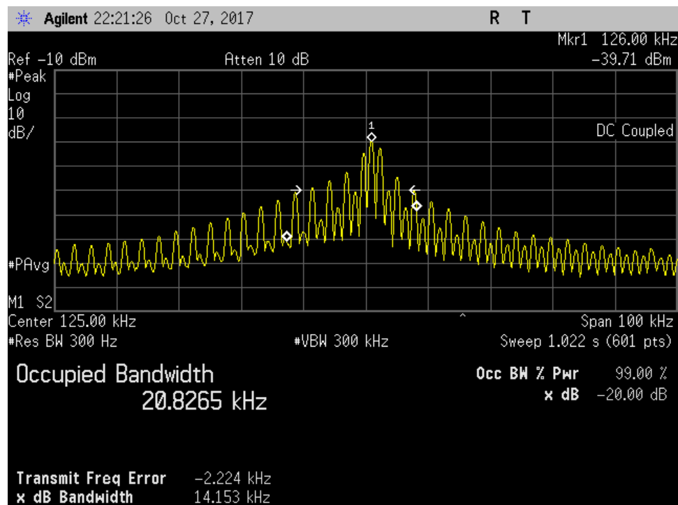
Figure 7.2.2-2: 99% BW
