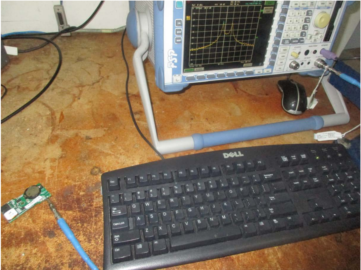
Figure 19: Occupied Bandwidth Measurements
