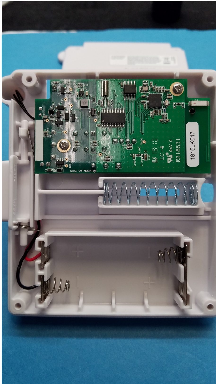
Figure 3: Assembled View
