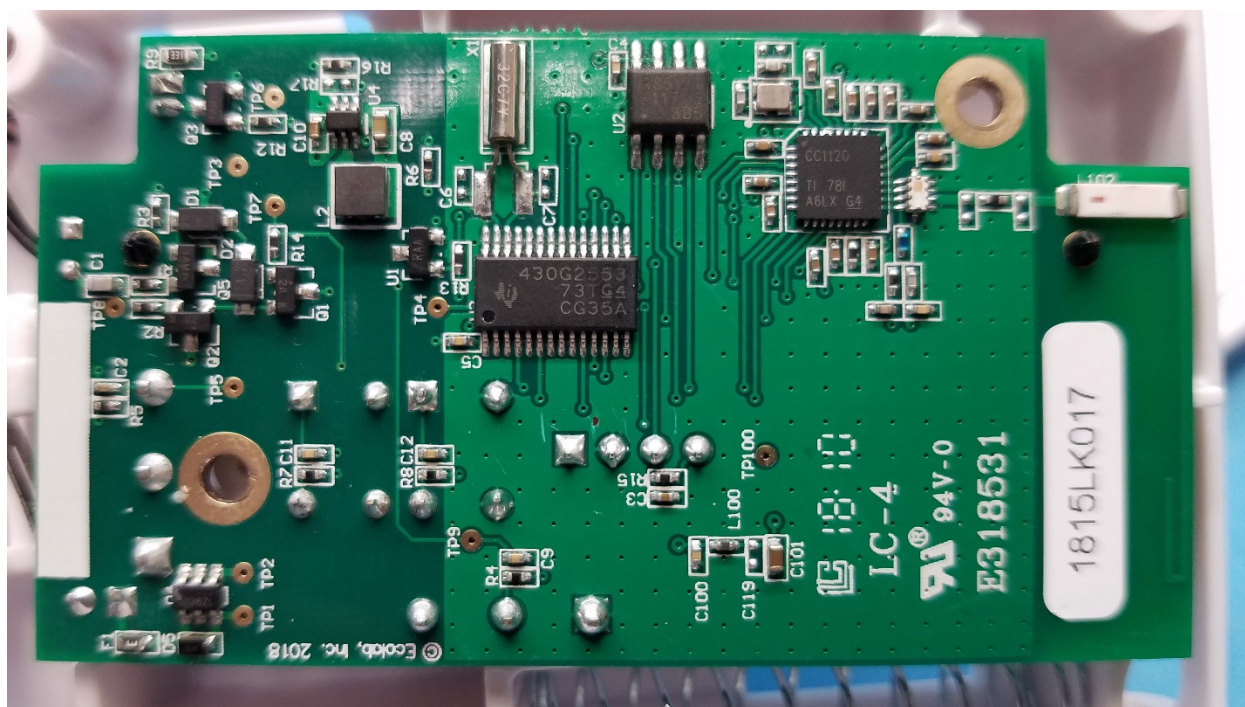
Figure 2: PCB Back
