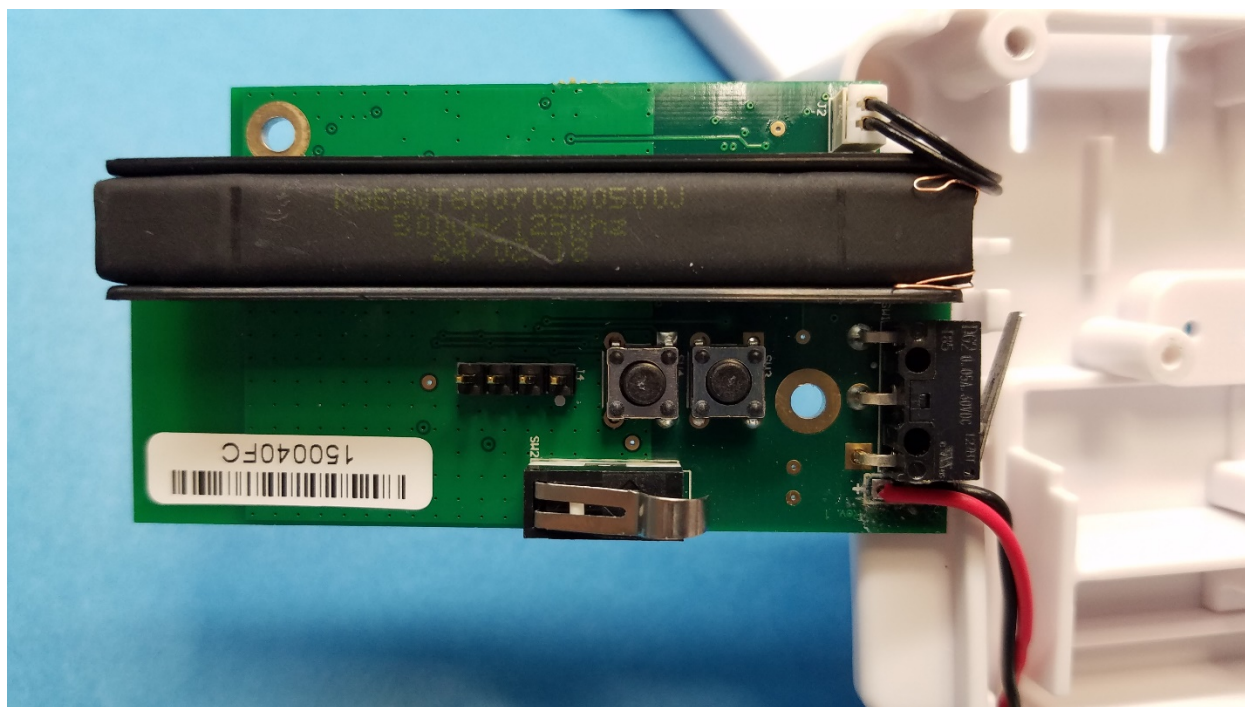
Figure 1: PCB Front
