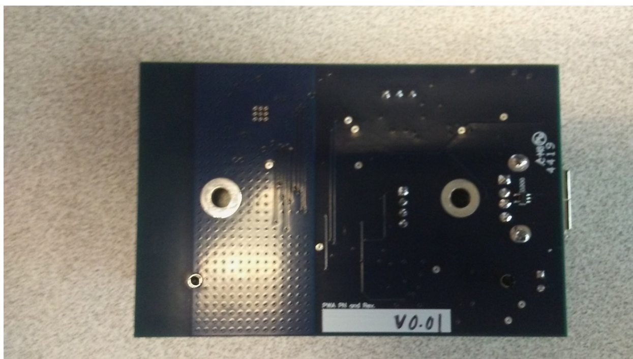
Figure 2: Bottom View
