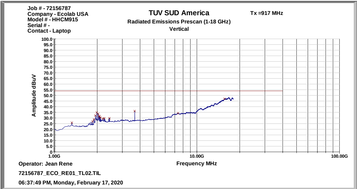
Figure 2.4.6-5: Radiated Emissions 1 GHz – 18 GHz – Vertical Polarization
