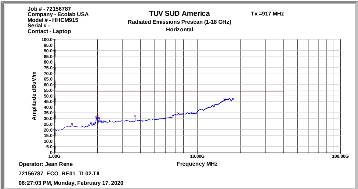
Figure 2.4.6-4: Radiated Emissions 1 GHz – 18 GHz – Horizontal Polarization
