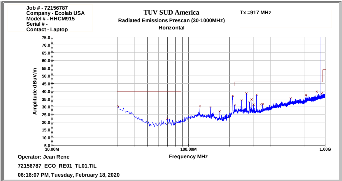
Figure 2.4.6-2: Radiated Emissions 30 MHz - 1 GHz – Horizontal Polarization
