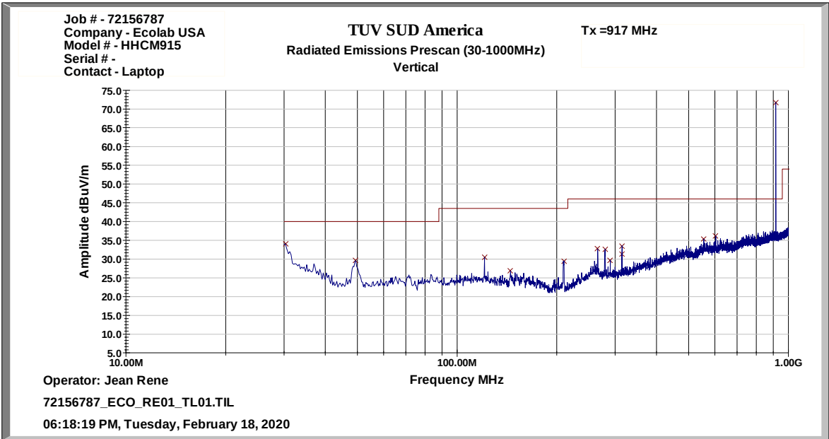
Figure 2.4.6-3: Radiated Emissions 30 MHz - 1 GHz – Vertical Polarization
