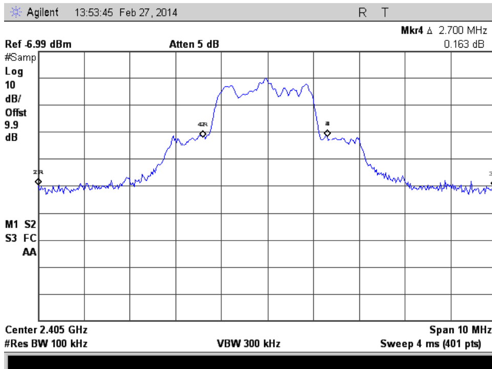
Figure 7.2.2-2: 99% OBW
