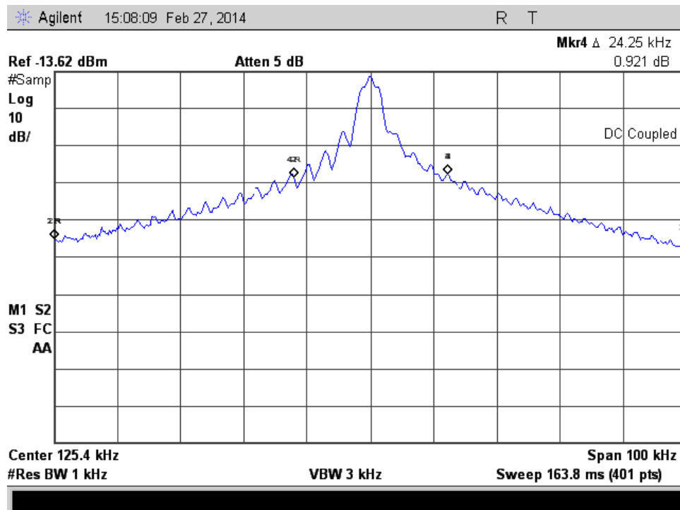
Figure 7.2.2-2: 99% OBW
