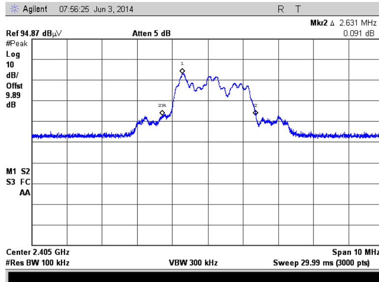
Figure 7.2.2-1: 20dB BW
