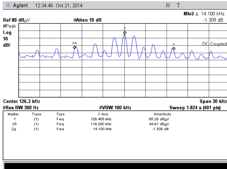
Figure 7.2.2-1: 20dB BW
