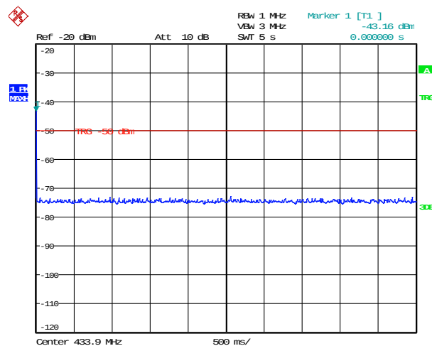
Figure 7.4.2-1: Periodic Operation
